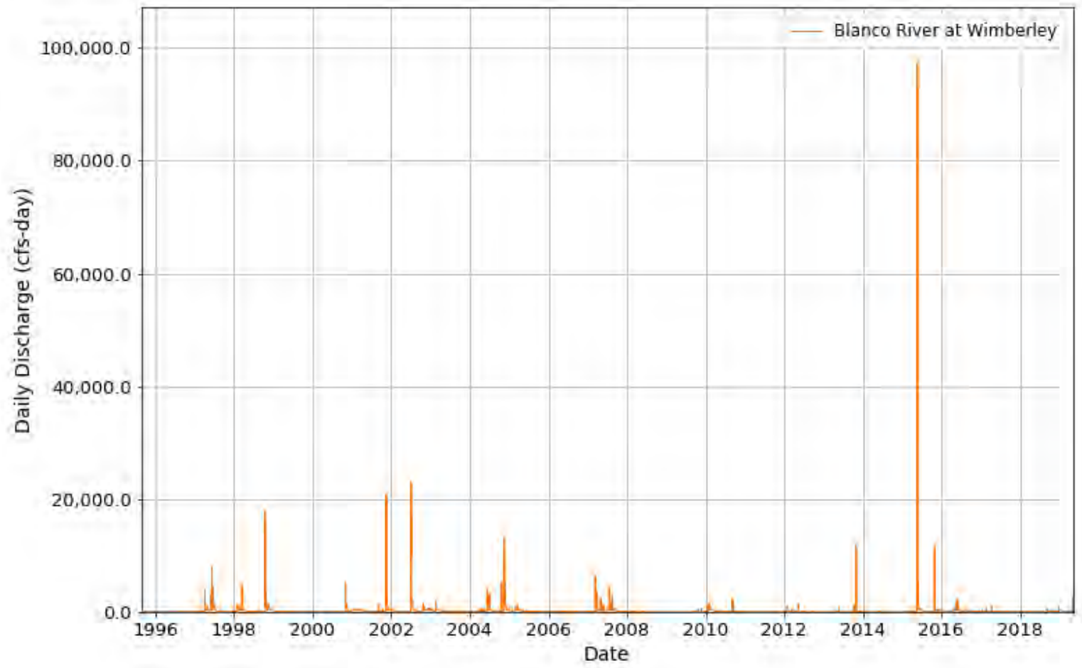
Figure 28: USGS 08171000 Blanco RR12- period of record hydrograph
