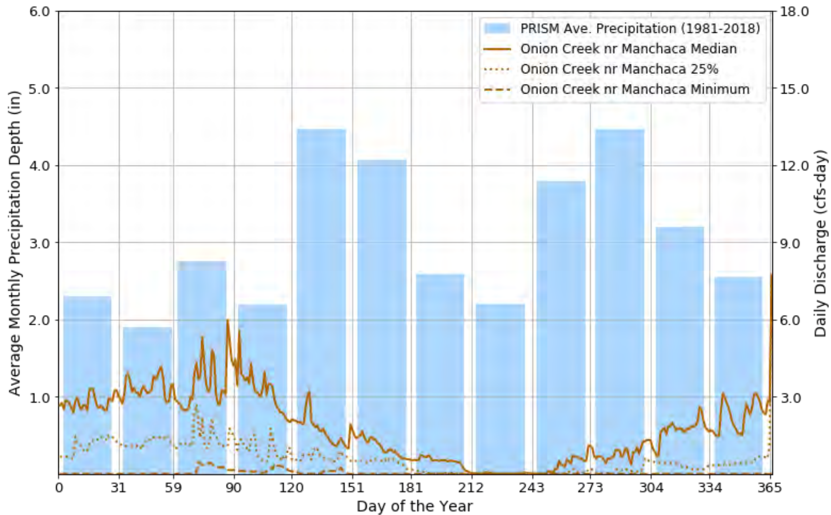
Figure 20: USGS 08158827 Onion Creek near Menchaca, TX - Median and low discharge summary
