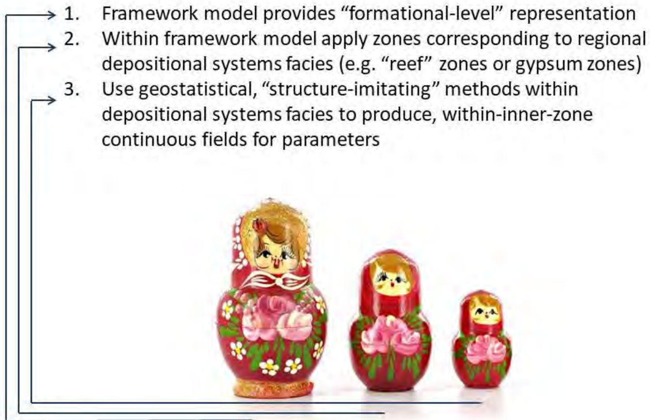
Figure 69: Conceptual description of nested groundwater model parameterization using a framework model
