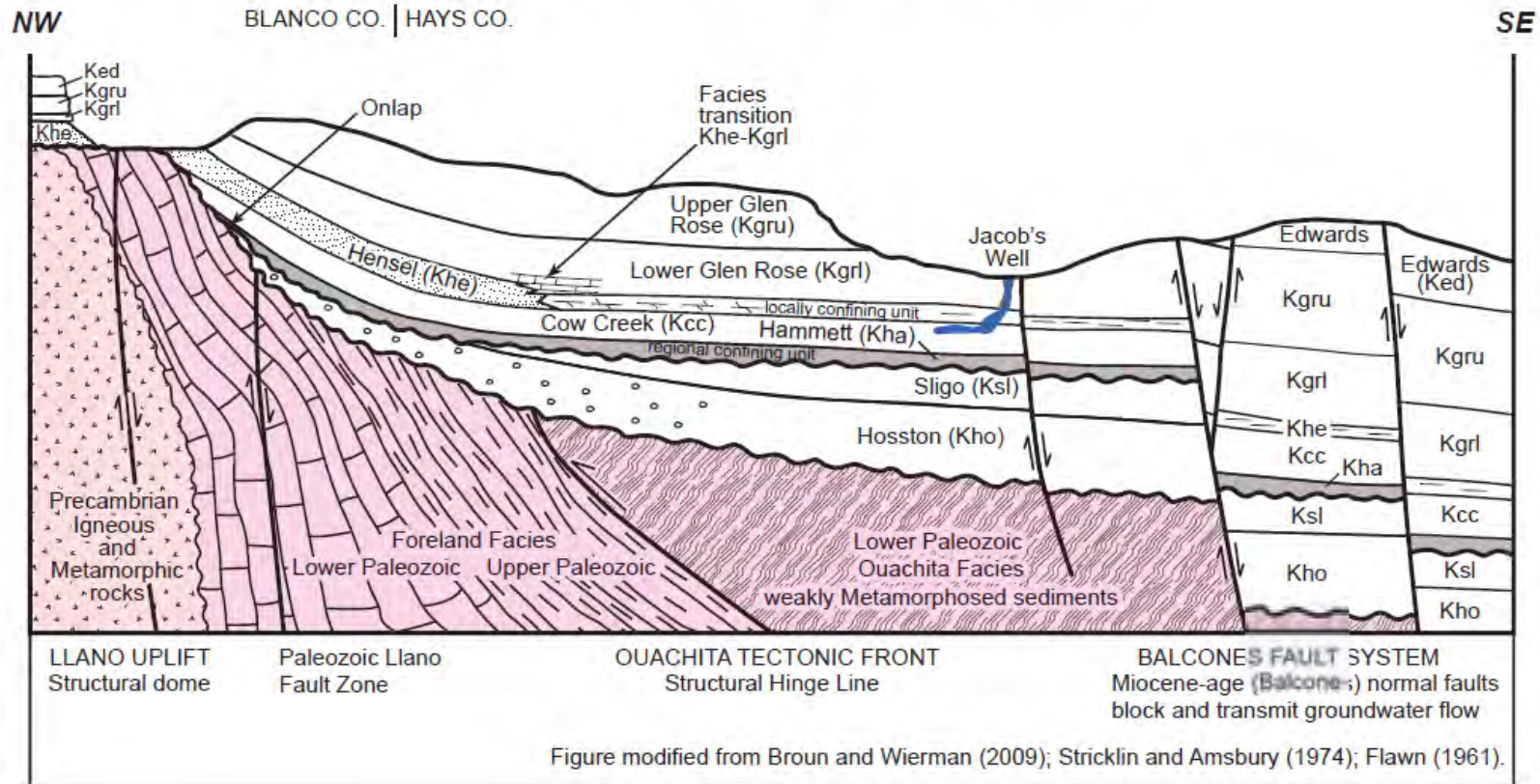
Figure 5: Structural control for Cretaceous (K) sedimentation, Figure 4-4 from Wierman et al. (2010)
