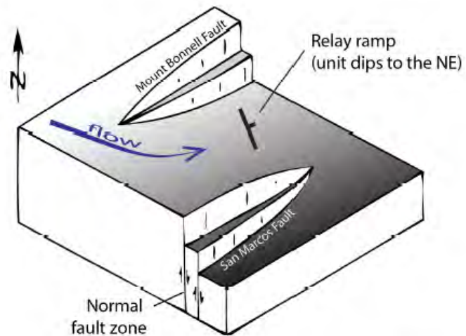
Figure 3. Schematic diagram of a relay ramp structure and its influence on groundwater flow. Two major faults transfer the displacement from one to the other resulting in folding, fracturing and faulting (not shown) along the ramp structure. These structures were proposed and mapped by Grimshaw and Woodruff (1986) and Collins and Hovorka (1997). Figure modified from Grimshaw and Woodruff (1986).
