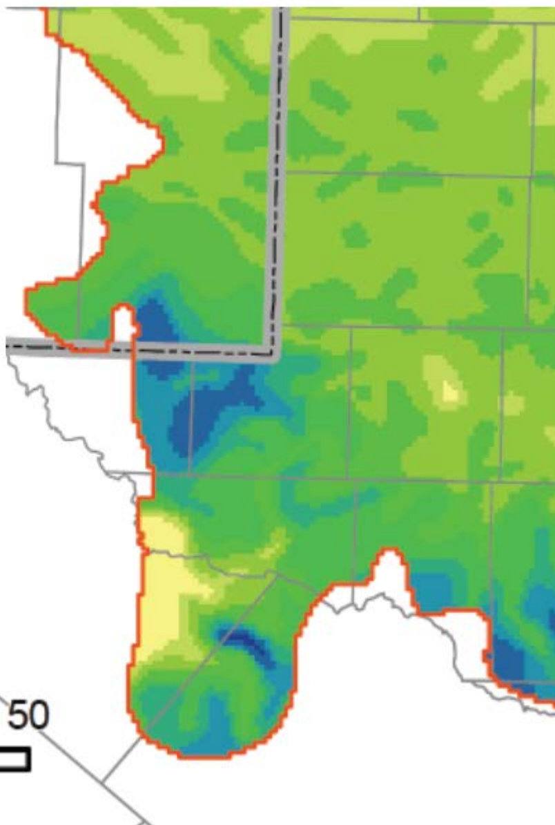
Figure 3.17: Sand fraction for the lower portion of the Dockum Group (modified from Ewing and others 2008).
