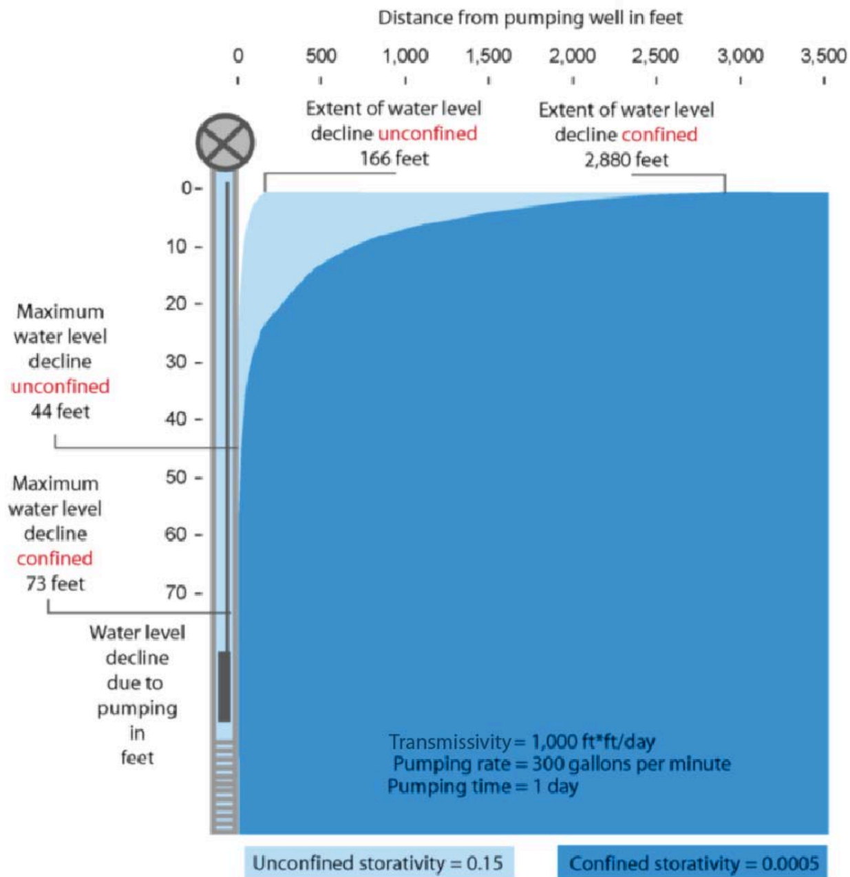
Figure 7.1: Comparison of water-level declines around a well in the exact same aquifer except that one is unconfined and one is confined. Aquifer properties shown are not meant to reflect those of the aquifers discussed in this study.
