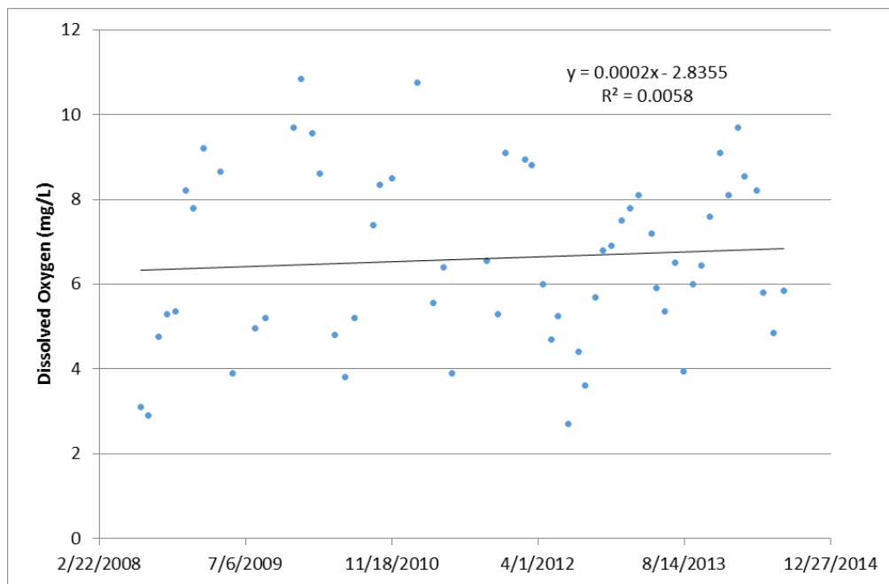
Figure 21: Dissolved Oxygen at site 80400
