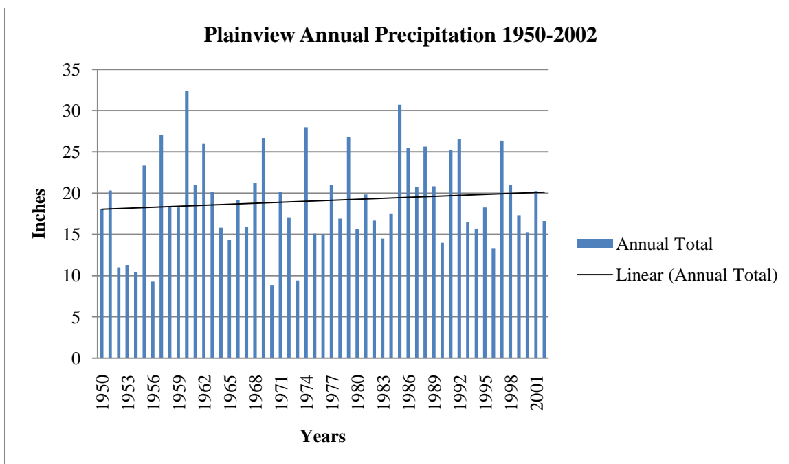
Figure 24. Plainview Annual Precipitation for the Period 1950-2002. Trend is not significant ( p = 0.435 ), b = 0.040 .
