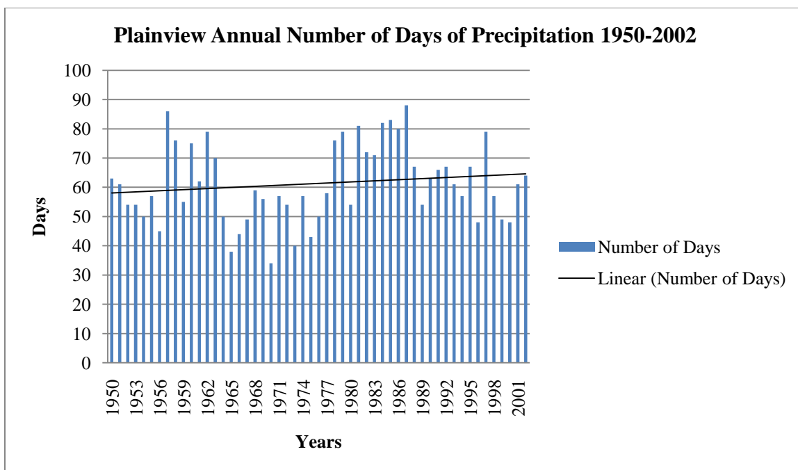
Figure 56. Plainview Annual Number of Days of Precipitation for the Period 1950-2002. Trend is not significant ( p = 0.290 ), b = 0.127 .
