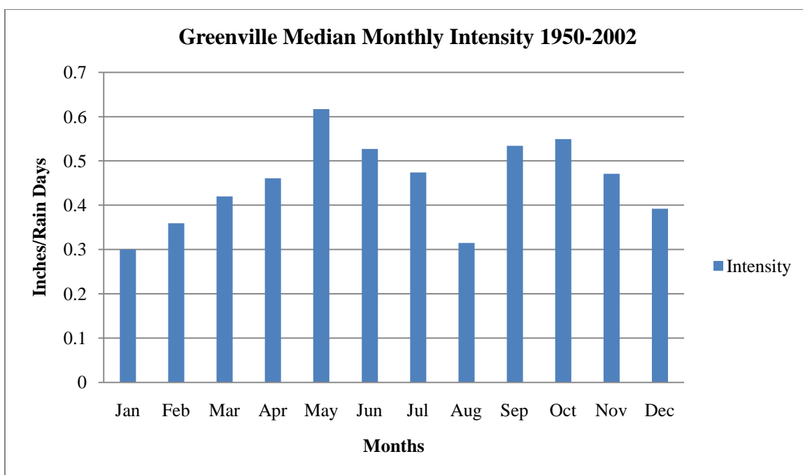
Figure 75. Greenville Median Monthly Intensity for the Period 1950-2002.
