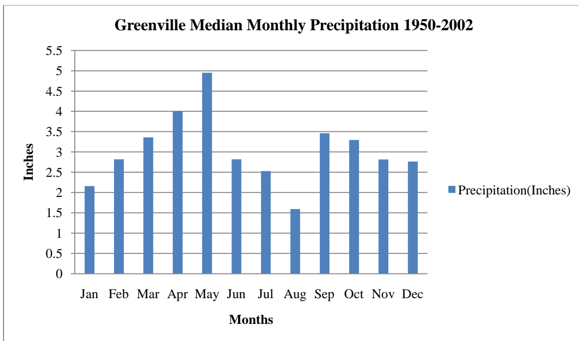
Figure 21. Greenville Median Monthly Precipitation for the Period 1950-2002.
