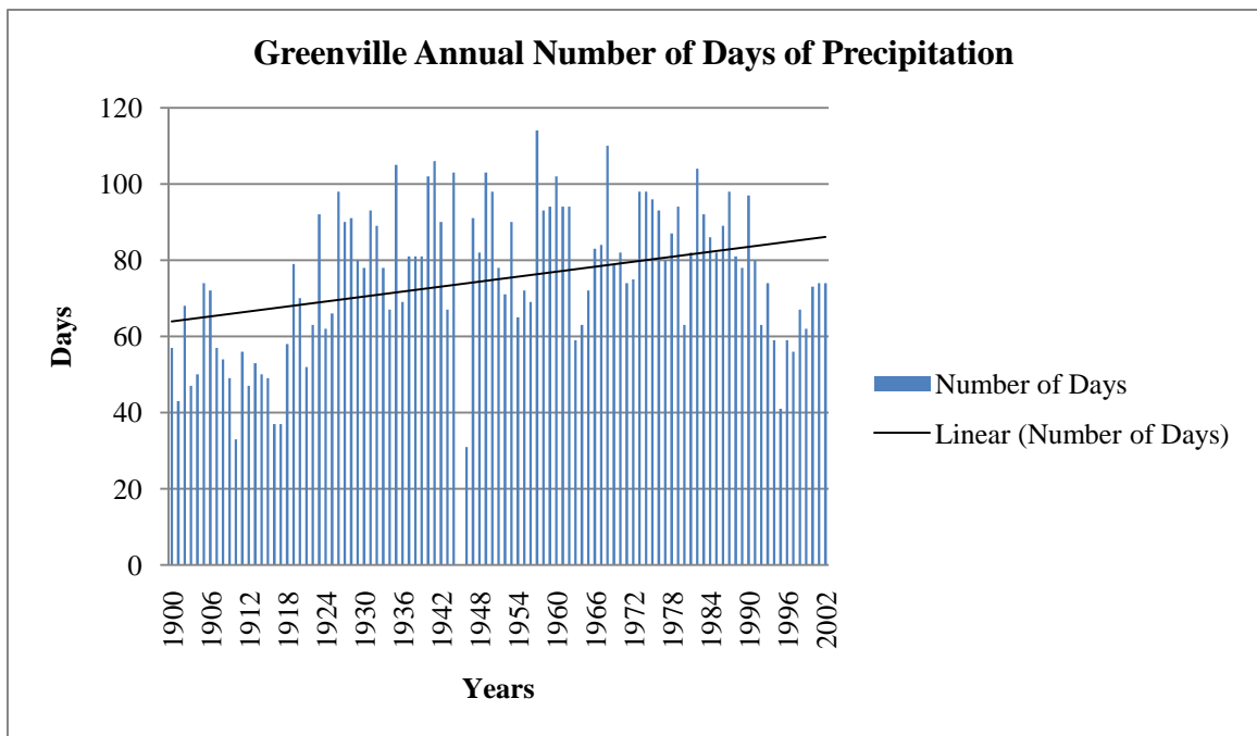
Figure 50. Greenville Annual Number of Days of Precipitation for the Period 1900-2002. Trend is significant ( p = 0.001 ), b = 0.218 .
