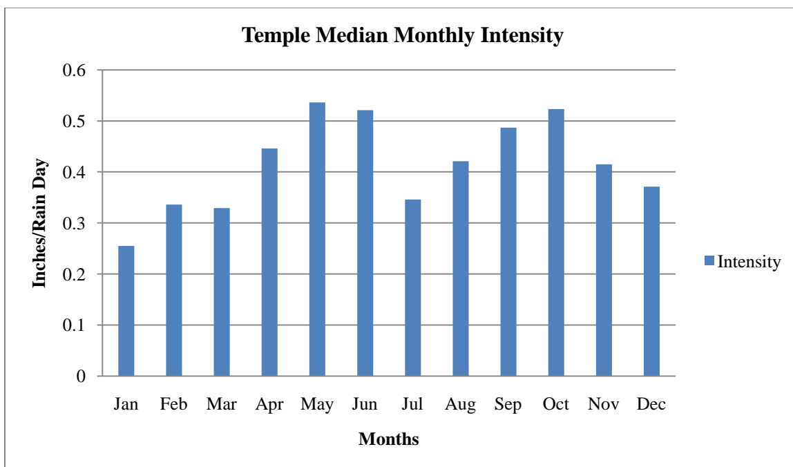
Figure 80. Temple Median Monthly Intensity for the Period 1897-2002.
