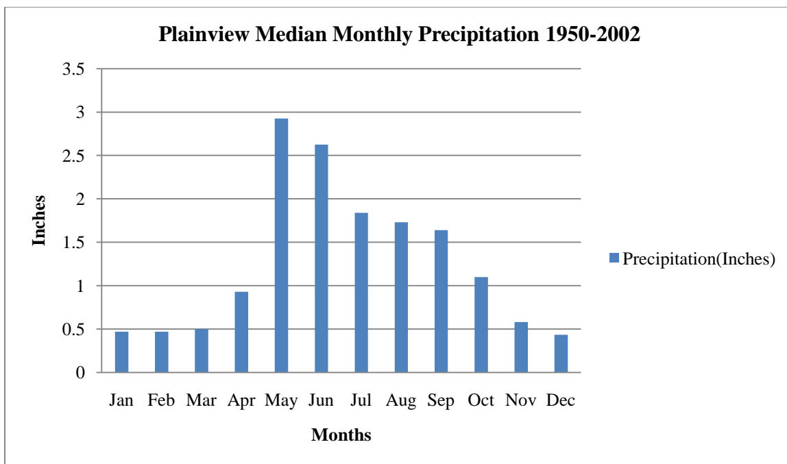
Figure 25. Plainview Median Monthly Precipitation for the Period 1950-2002.
