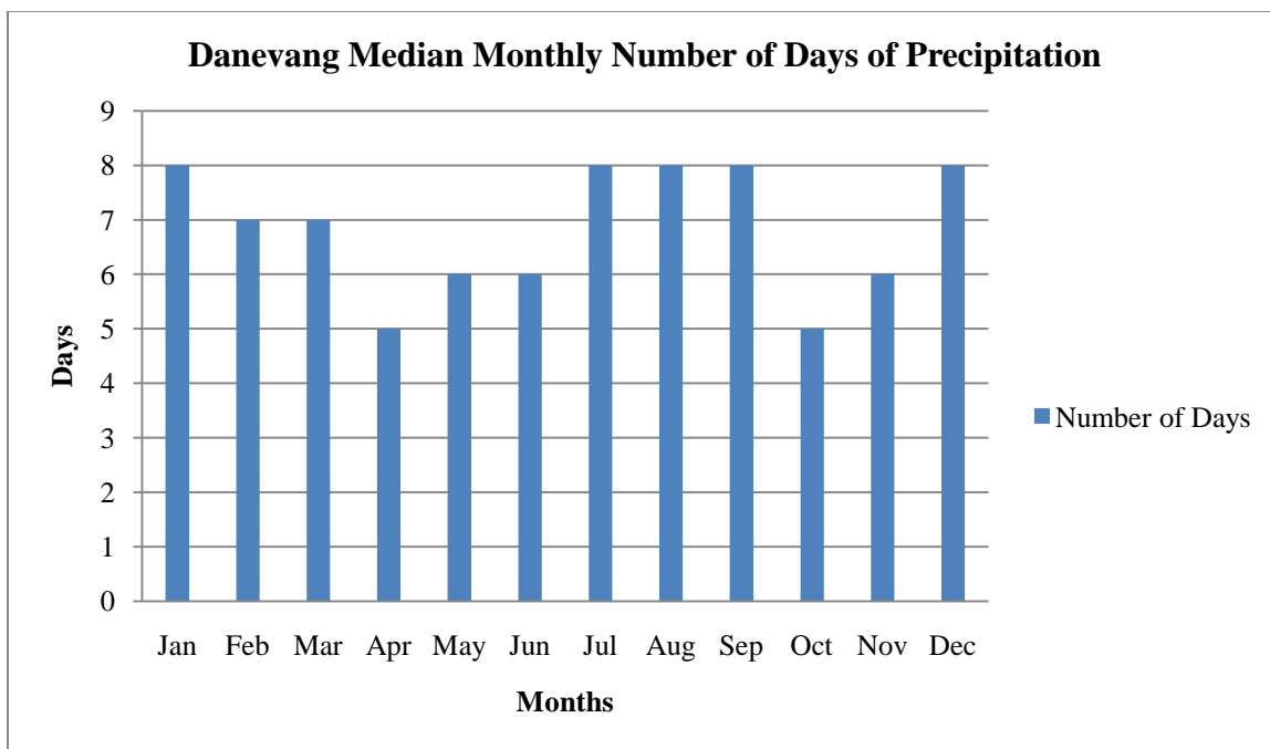
Figure 47. Danevang Median Monthly Number of Days of Precipitation for the Period 1897-2002.
