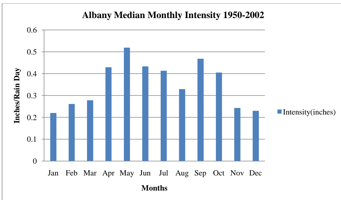
Figure 67. Albany Median Monthly Intensity for the Period 1901-2002.
