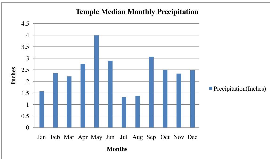
Figure 31. Temple Median Monthly Precipitation for the Period 1897-2002.
