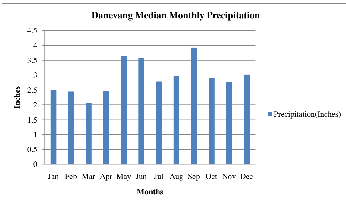
Figure 15. Danevang Median Monthly Precipitation for the Period 1897-2002.
