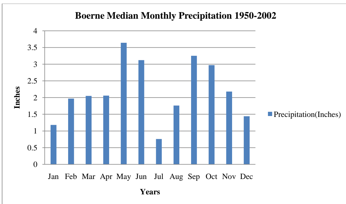
Figure 13. Boerne Median Monthly Precipitation for the Period 1950-2002.
