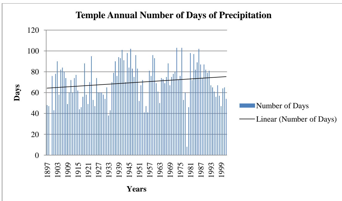
Figure 62. Temple Annual Number of Days of Precipitation for the Period 1897-2002. Trend is significant ( p = 0.081 ), b = 0.105 .
