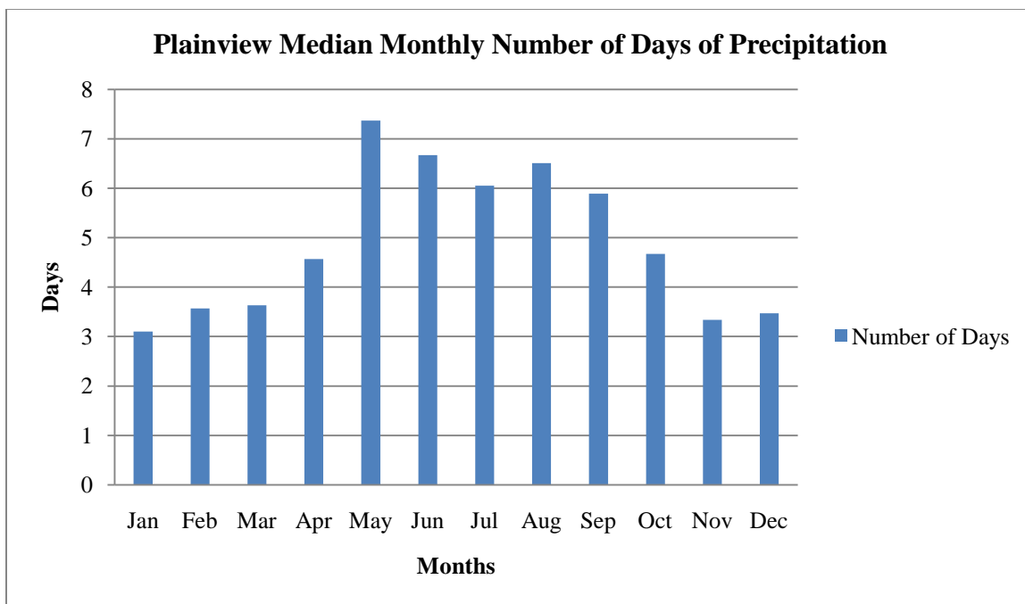
Figure 55. Plainview Median Monthly Number of Days of Precipitation for the Period 1950-2002.
