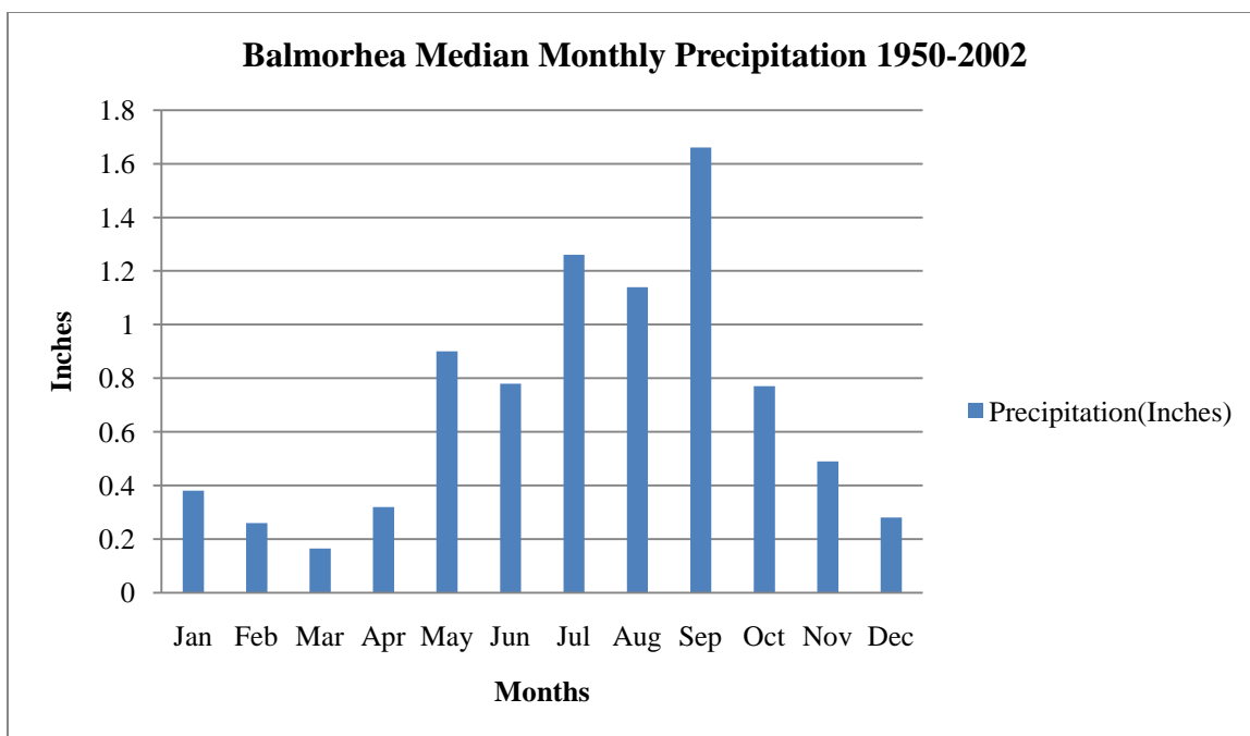
Figure 9. Balmorhea Median Monthly Precipitation for the Period 1950-2002.
