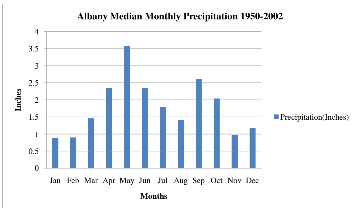
Figure 5. Albany Median Monthly Precipitation for the Period 1950-2002.
