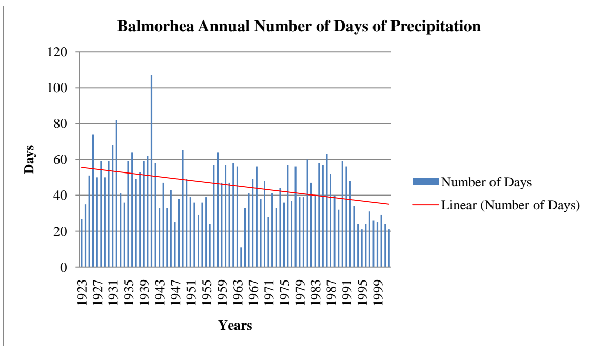
Figure 38. Balmorhea Annual Number of Days of Precipitation for the Period 1923-2002. Trend is significant ( p = 0.000 ), b = -0.259 .
