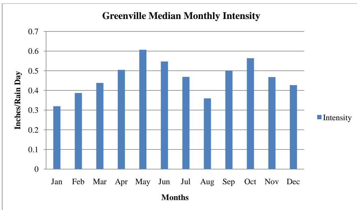
Figure 74. Greenville Median Monthly Intensity for the Period 1900-2002.
