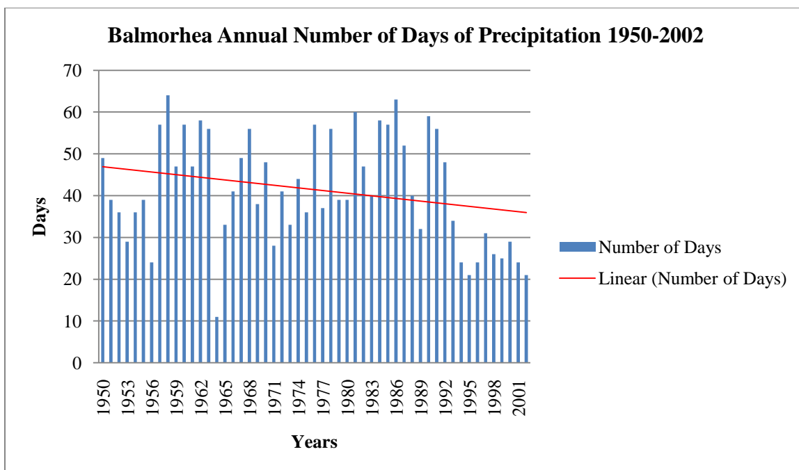
Figure 40. Balmorhea Annual Number of Days of Precipitation for the Period 1950-2002. Trend is significant ( p = 0.073 ), b = -0.211 .
