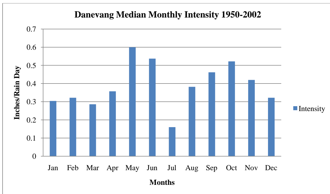
Figure 73. Danevang Median Monthly Intensity for the Period 1950-2002.
