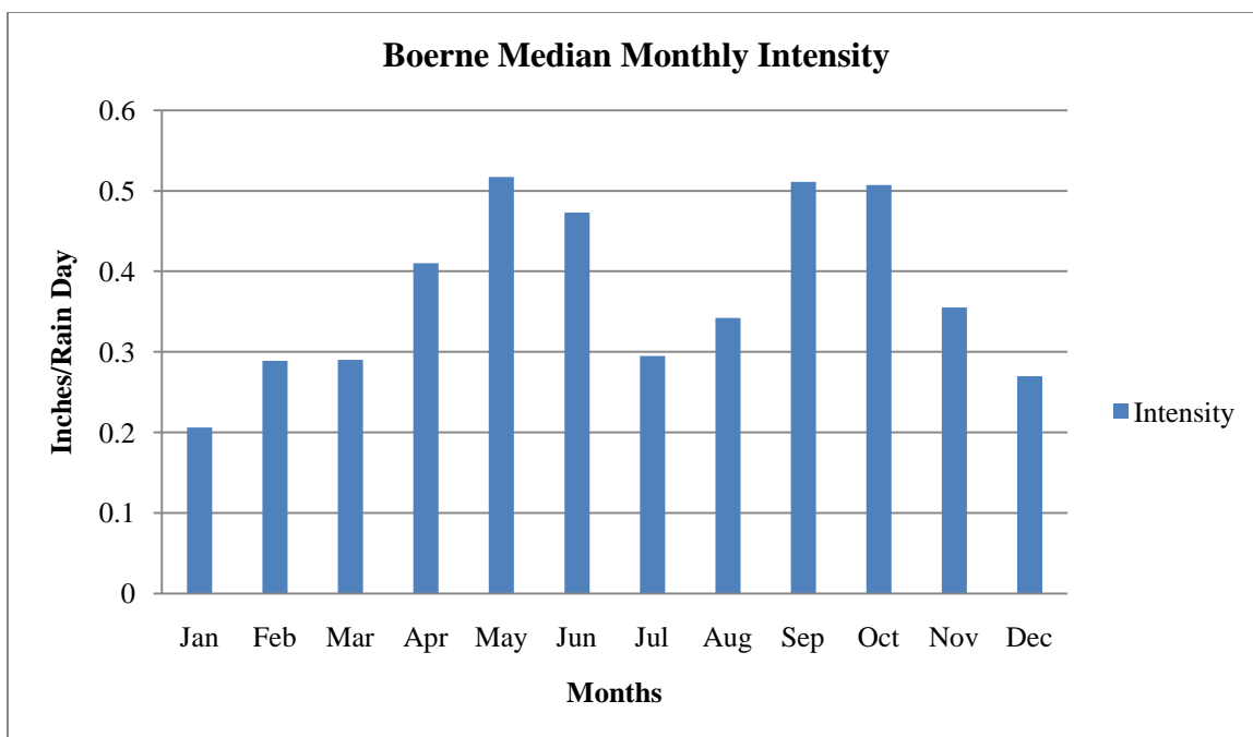
Figure 70. Boerne Median Monthly Intensity for the Period 1897-2002.
