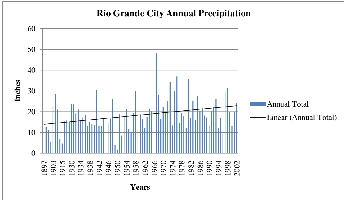
Figure 26. Rio Grande City Annual Precipitation for the Period 1897-2002. Trend is significant ( p = 0.002 ), b = 0.095 .
