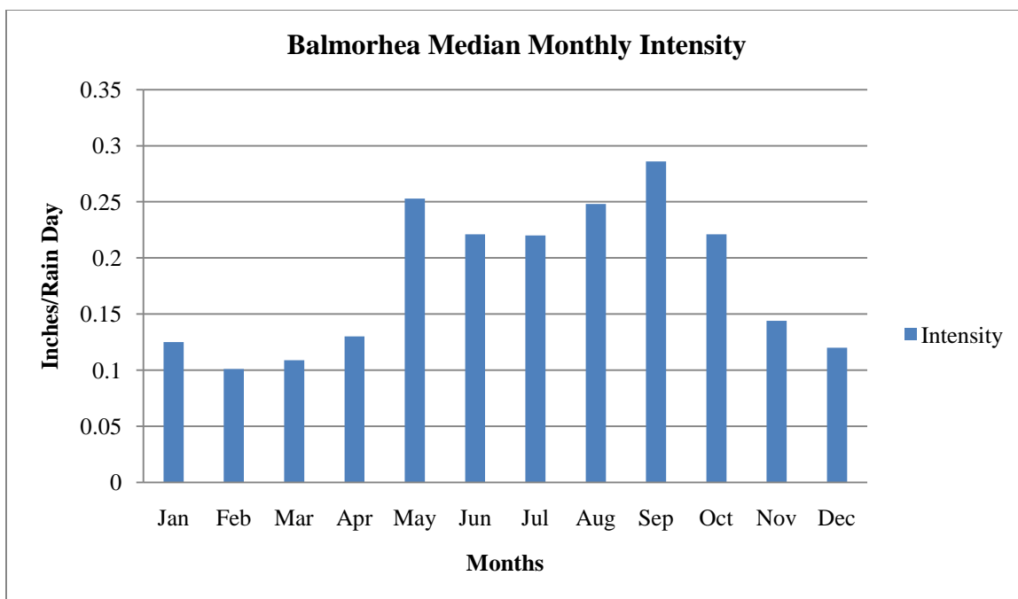
Figure 68. Balmorhea Median Monthly Intensity for the Period 1923-2002.
