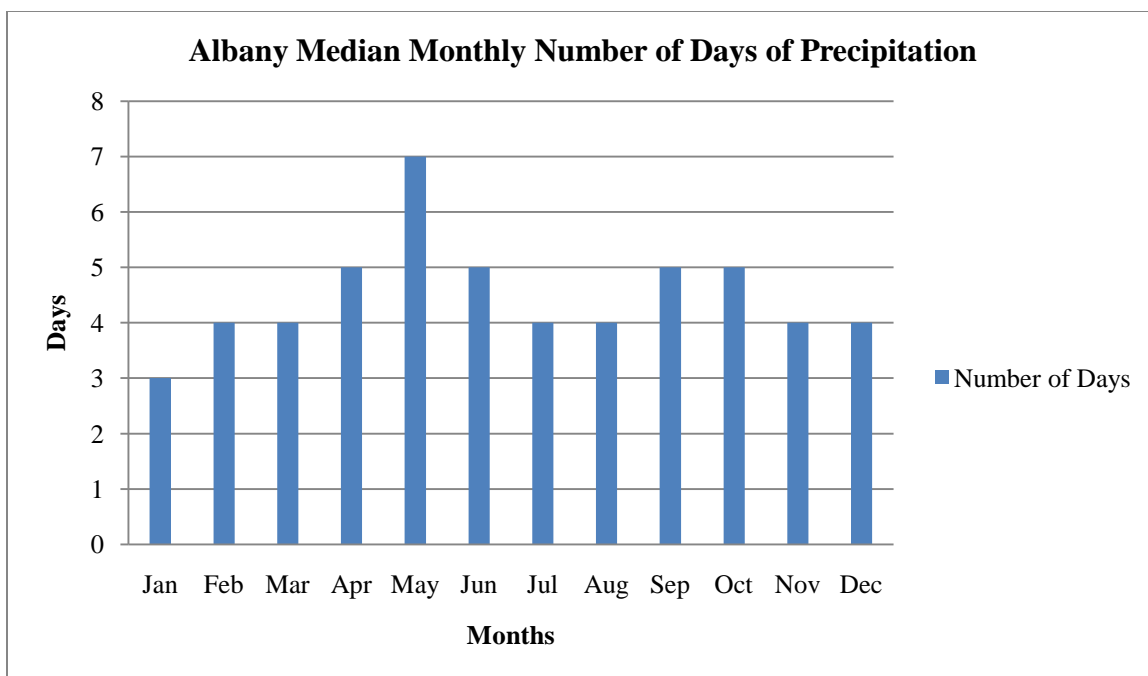
Figure 35. Albany Median Monthly Number of Days of Precipitation for the Period 1901-2002.
