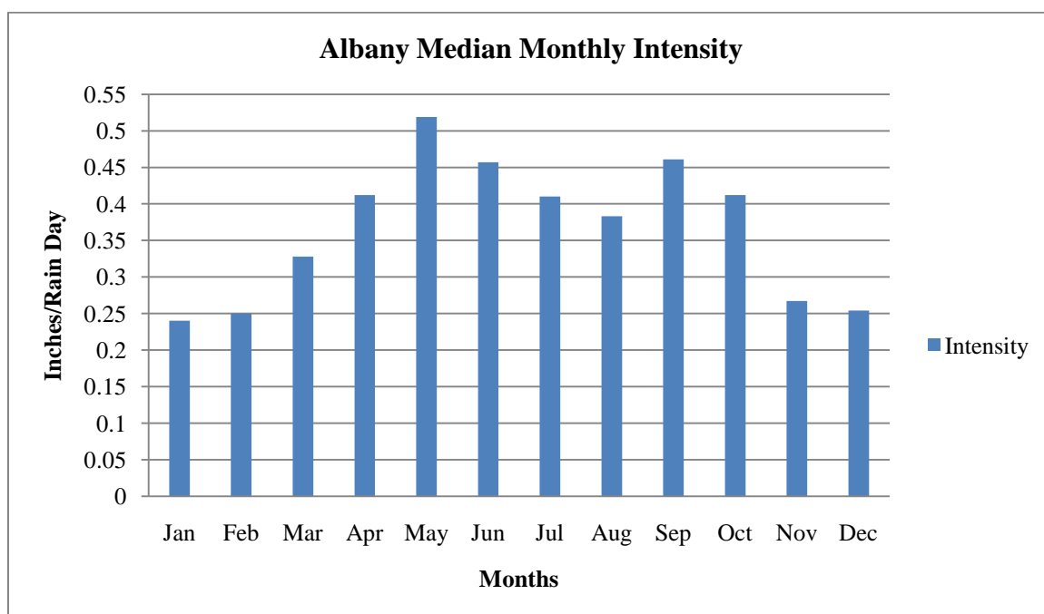
Figure 66. Albany Median Monthly Intensity for the Period 1901-2002.
