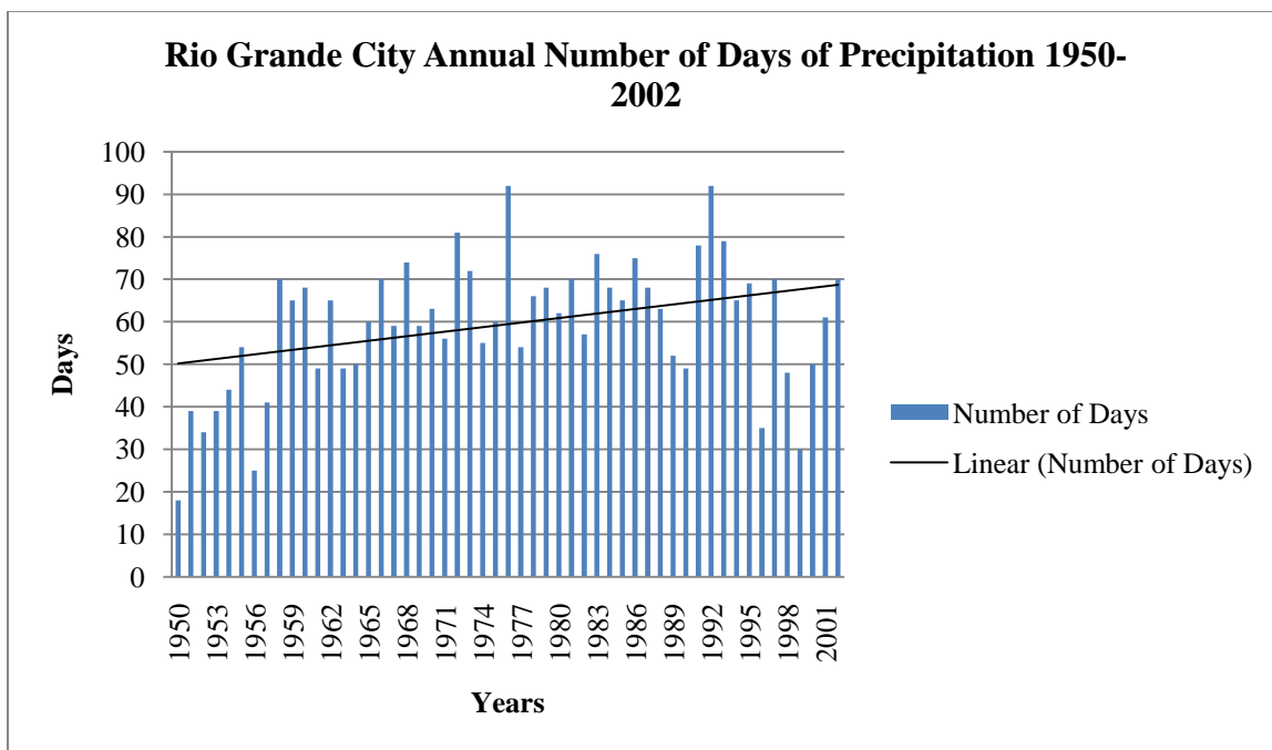
Figure 60. Rio Grande City Annual Number of Days of Precipitation for the Period 1950-2002. Trend is significant ( p = 0.010 ), b = 0.355 .
