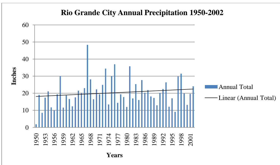
Figure 28. Rio Grande City Annual Precipitation for the Period 1950-2002. Trend is not significant ( p = 0.264 ), b = 0.083 .
