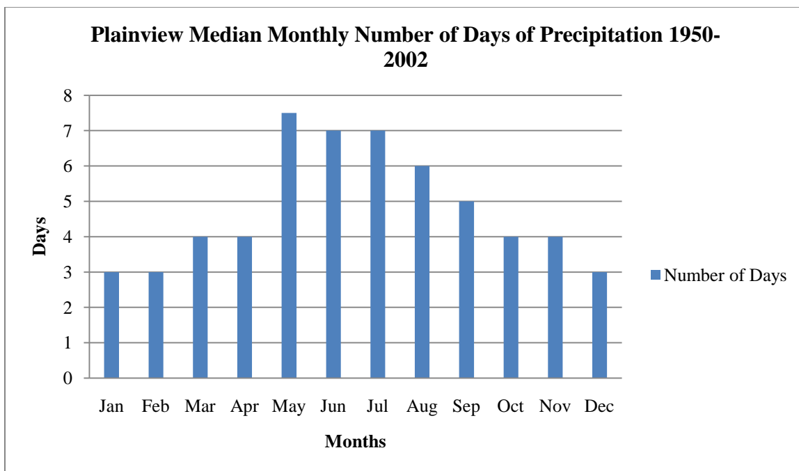
Figure 57. Plainview Median Monthly Number of Days of Precipitation for the Period 1950-2002.
