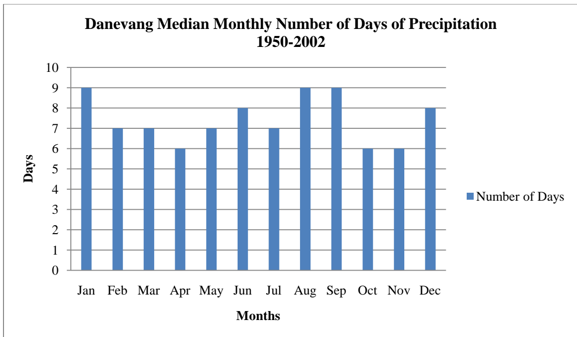
Figure 49. Danevang Median Monthly Number of Days of Precipitation for the Period 1950-2002.
