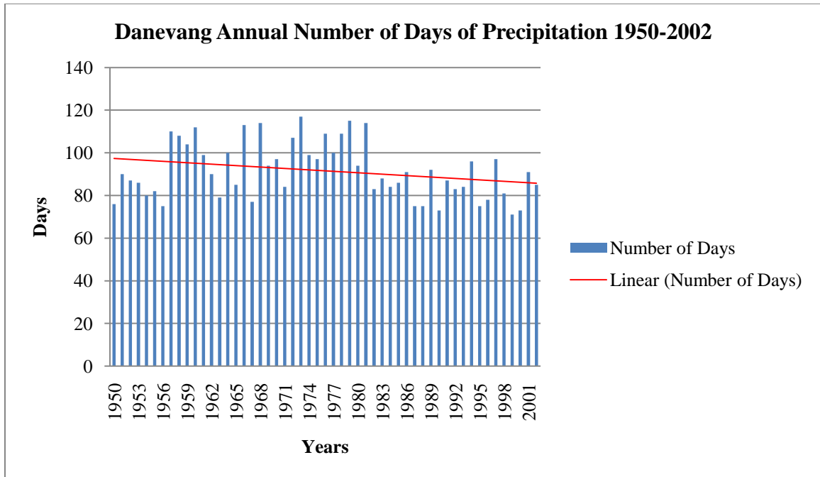
Figure 48. Danevang Annual Number of Days of Precipitation for the Period 1950-2002. Trend is significant ( p = 0.058 ), b = -0.222 .
