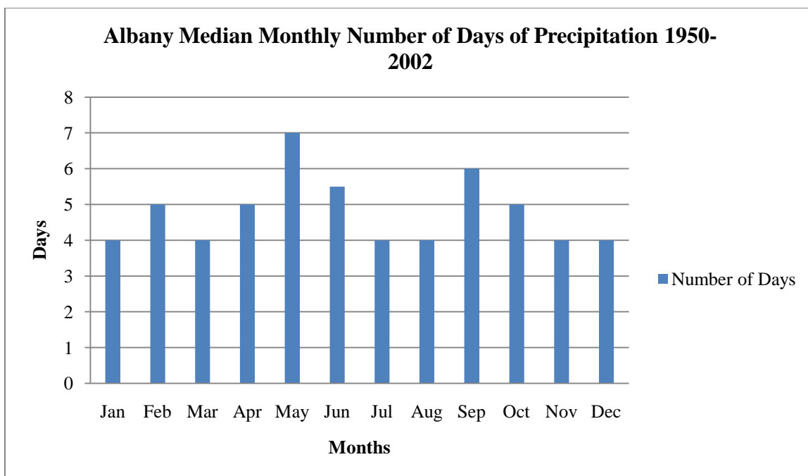
Figure 37. Albany Median Monthly Number of Days of Precipitation for the Period 1950-2002.
