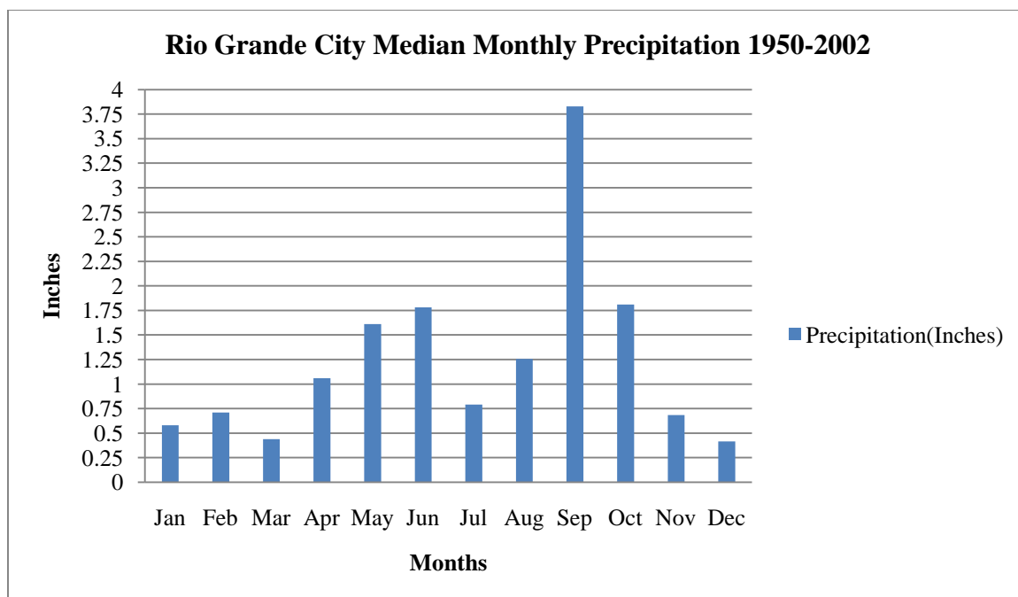
Figure 29. Rio Grande City Median Monthly Precipitation for the Period 1950-2002.
