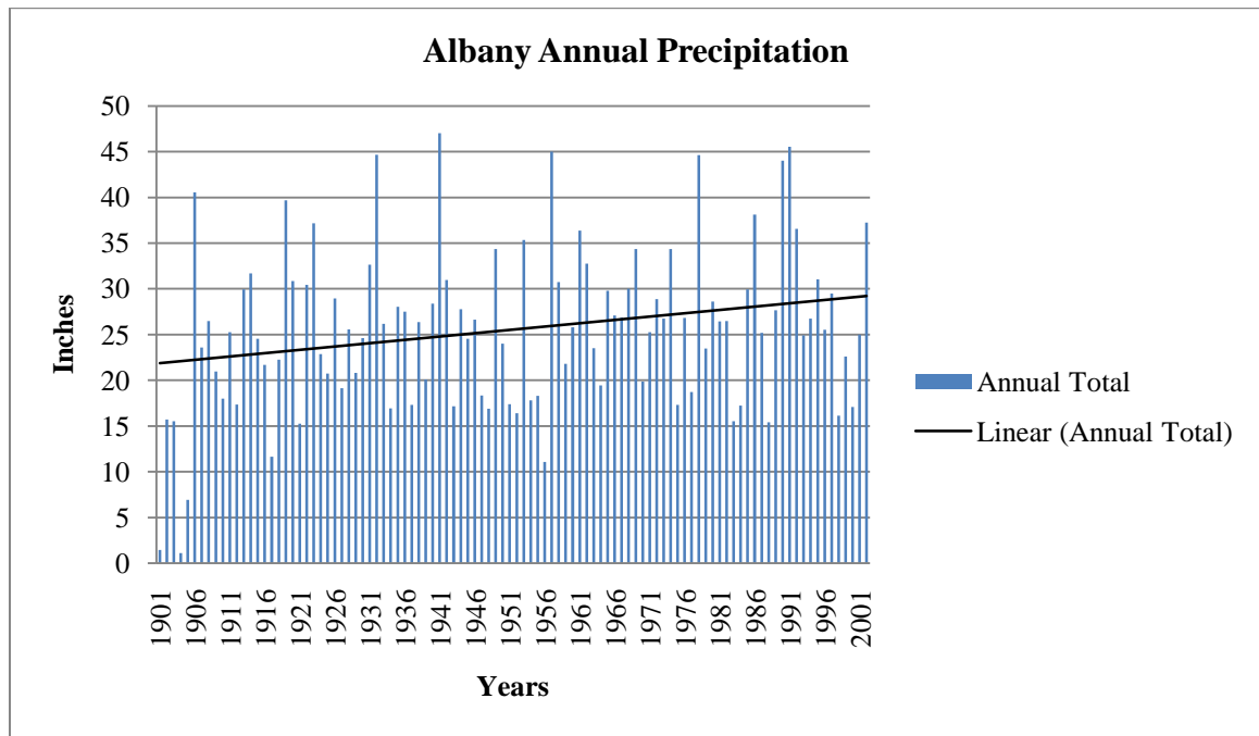
Figure 2. Albany Annual Precipitation for the Period 1901-2002. Trend is significant ( p = 0.014 ), b = 0.073 .
