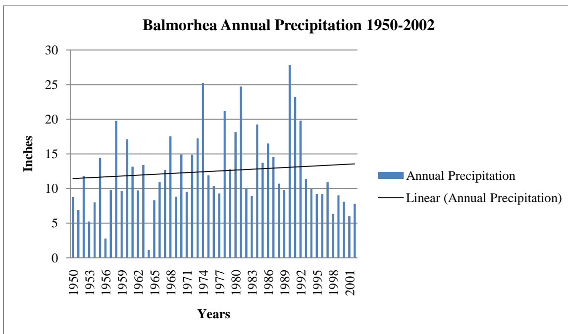
Figure 8. Balmorhea Annual Precipitation for the Period 1950-2002. Trend is not significant ( p = 0.423 ), b = 0.041 .
