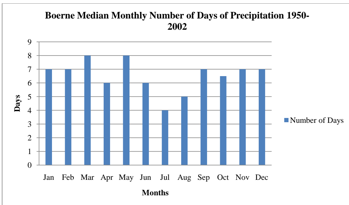
Figure 45. Boerne Median Monthly Number of Days of Precipitation for the Period 1950-2002.
