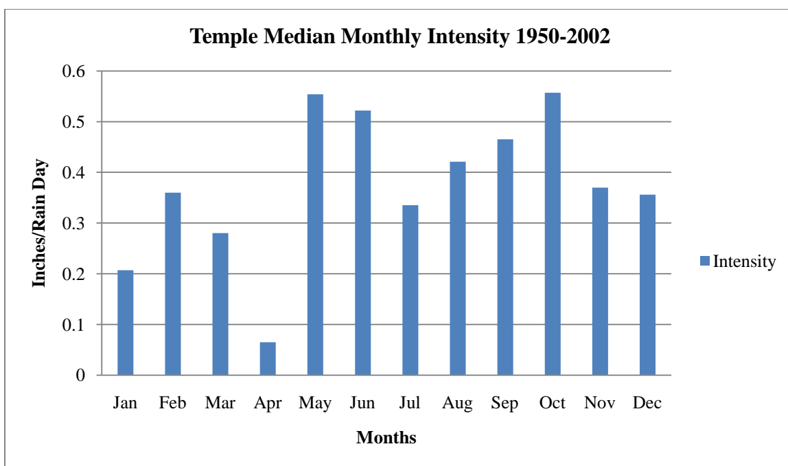
Figure 81. Temple Median Monthly Intensity for the Period 1950-2002.
