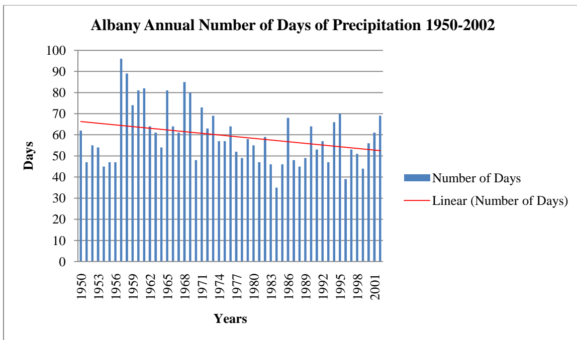
Figure 36. Albany Annual Number of Days of Precipitation for the Period 1950-2002. Trend is significant ( p = 0.026 ), b = -0.264 .
