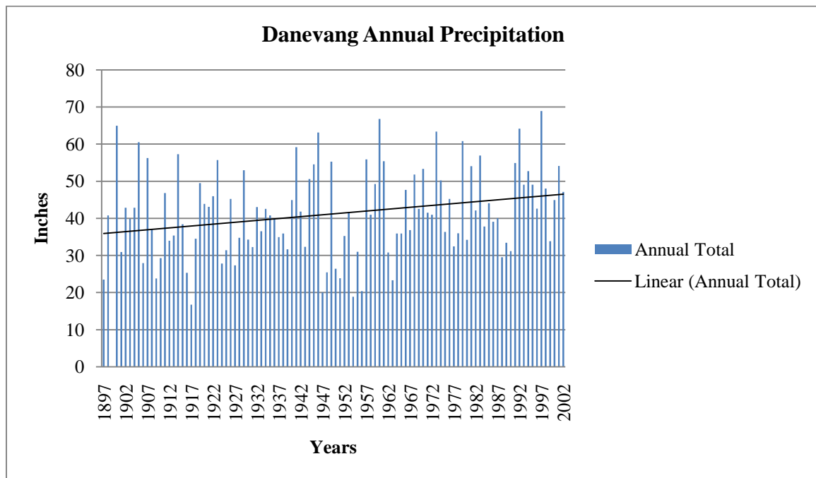
Figure 14. Danevang Annual Precipitation for the Period 1897-2002. Trend is significant ( p = 0.009 ), b = 0.101 .
