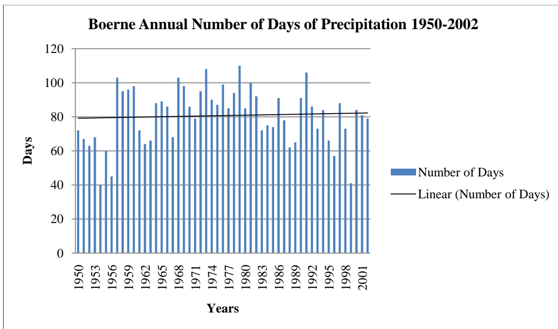
Figure 44. Boerne Annual Number of Days of Precipitation for the Period 1950-2002. Trend is not significant ( p = 0.693 ), b = 0.060 .
