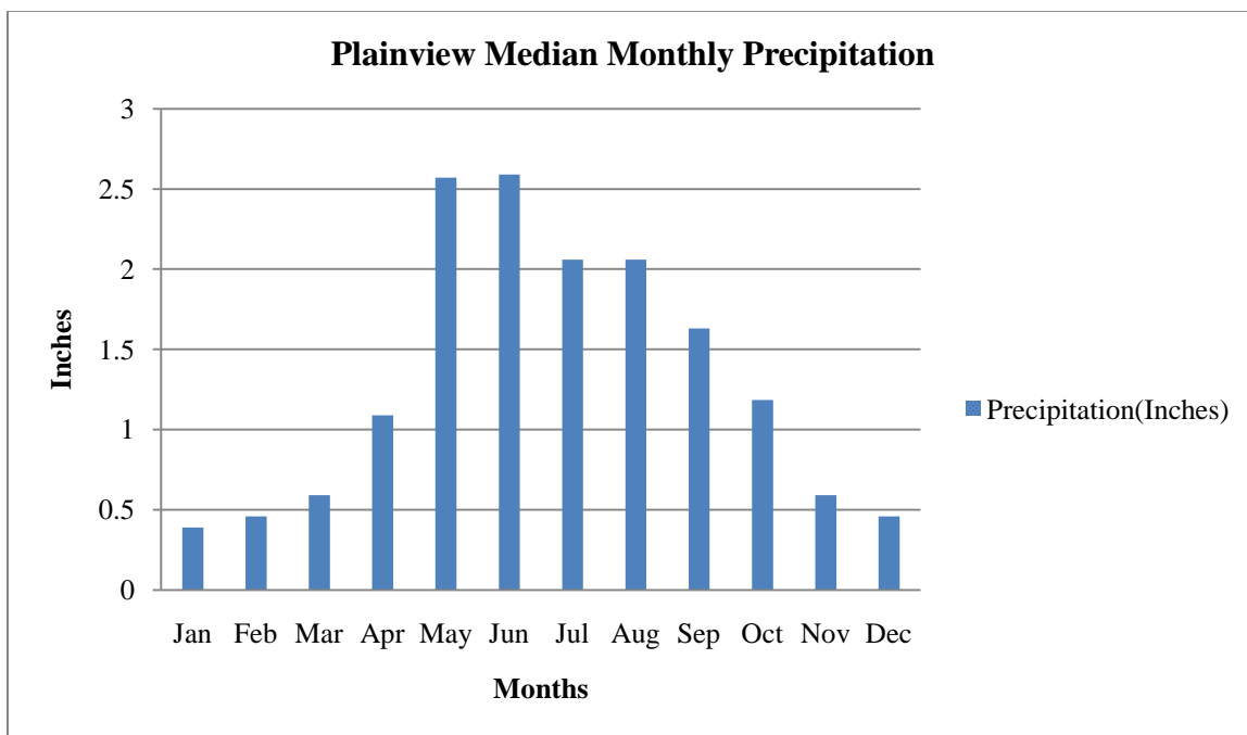
Figure 23. Plainview Median Monthly Precipitation for the Period 1908-2002.
