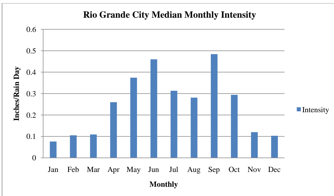
Figure 78. Rio Grande City Median Monthly Intensity for the Period 1897-2002.
