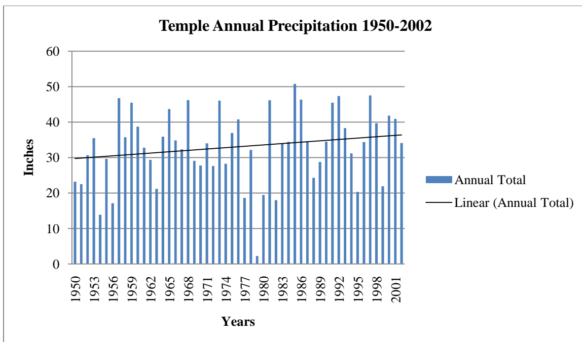
Figure 32. Temple Annual Precipitation for the Period 1950-2002. Trend is not significant ( p = 0.165 ), b = 0.128 .
