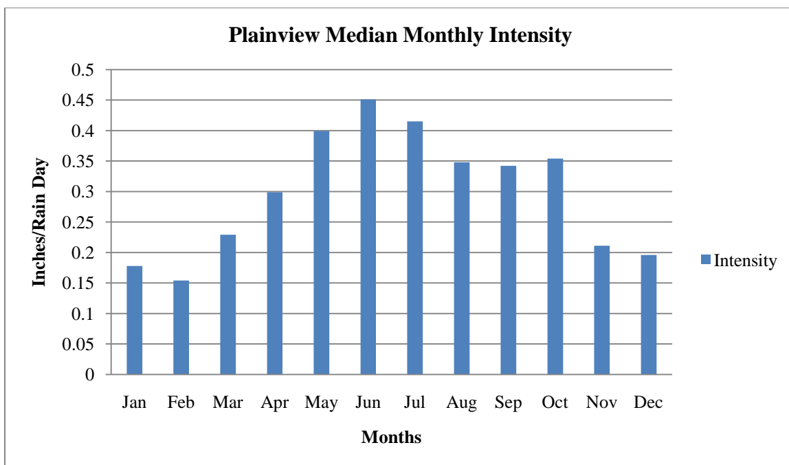
Figure 76. Plainview Median Monthly Intensity for the Period 1908-2002.
