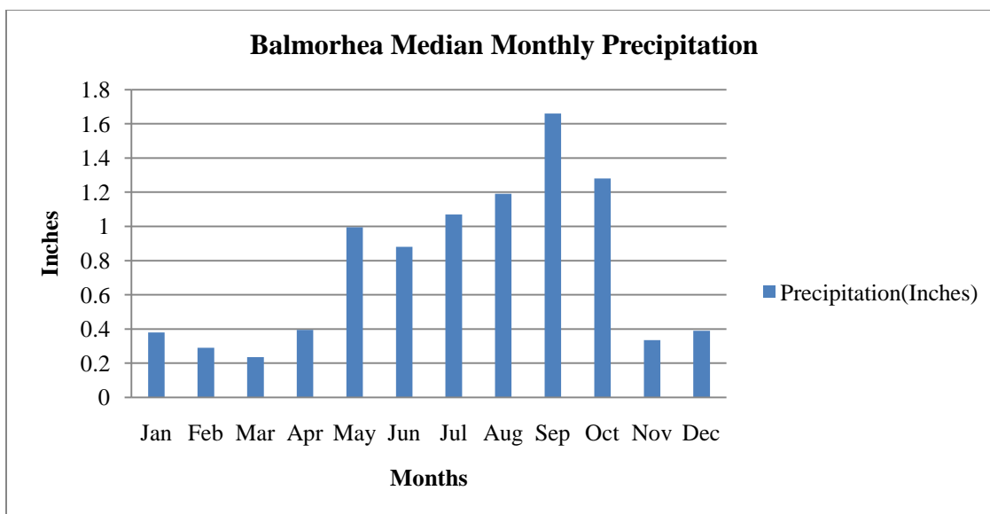
Figure 7. Balmorhea Median Monthly Precipitation for the Period 1923-2002.
