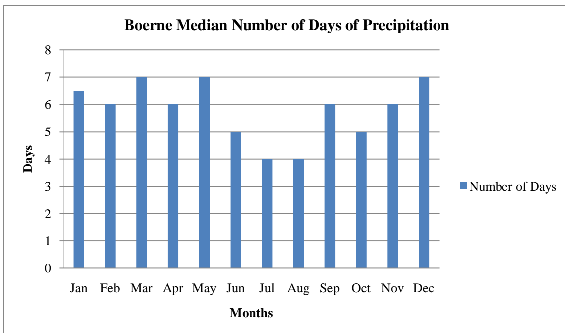
Figure 43. Boerne Median Monthly Number of Days of Precipitation for the Period 1897-2002.
