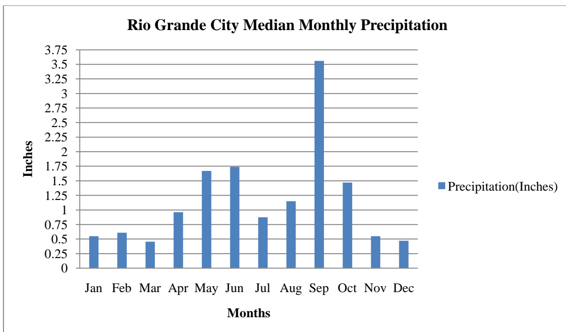
Figure 27. Rio Grande City Median Monthly Precipitation for the Period 1897-2002.
