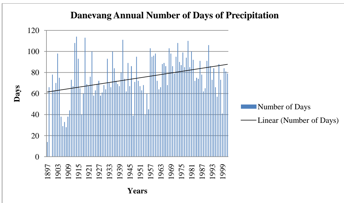
Figure 46. Danevang Annual Number of Days of Precipitation for the Period 1897-2002. Trend is significant ( p = 0.000 ), b = 0.250 .
