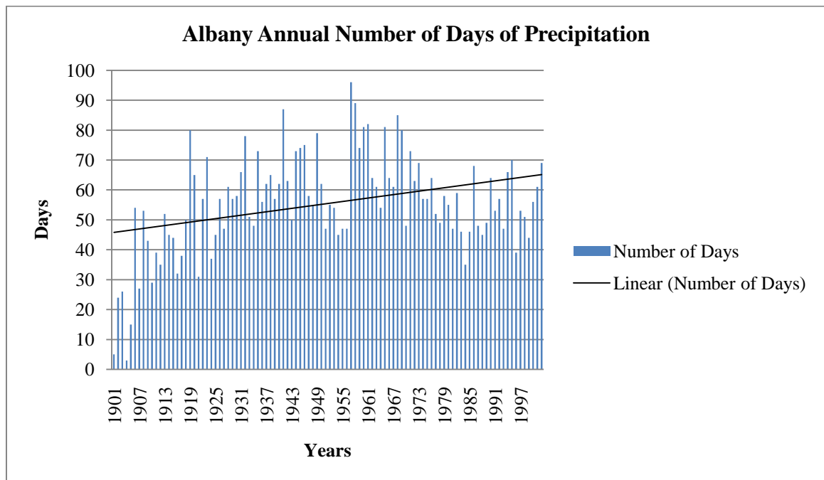
Figure 34. Albany Annual Number of Days of Precipitation for the Period 1901-2002. Trend is significant ( p = 0.001 ), b = 0.191 .
