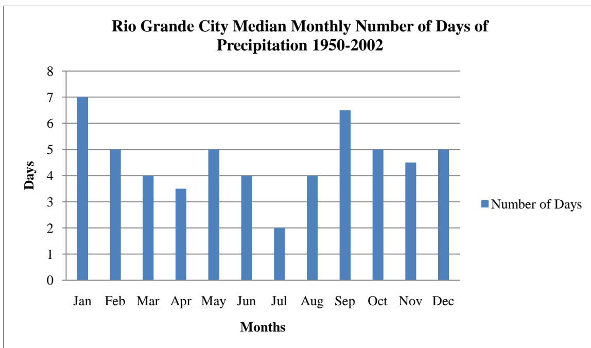
Figure 61. Rio Grande City Median Monthly Number of Days of Precipitation for the Period 1950-2002.
