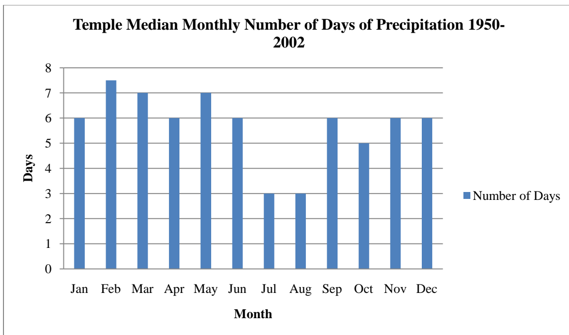
Figure 65. Temple Median Monthly Number of Days of Precipitation for the Period 1950-2002.
