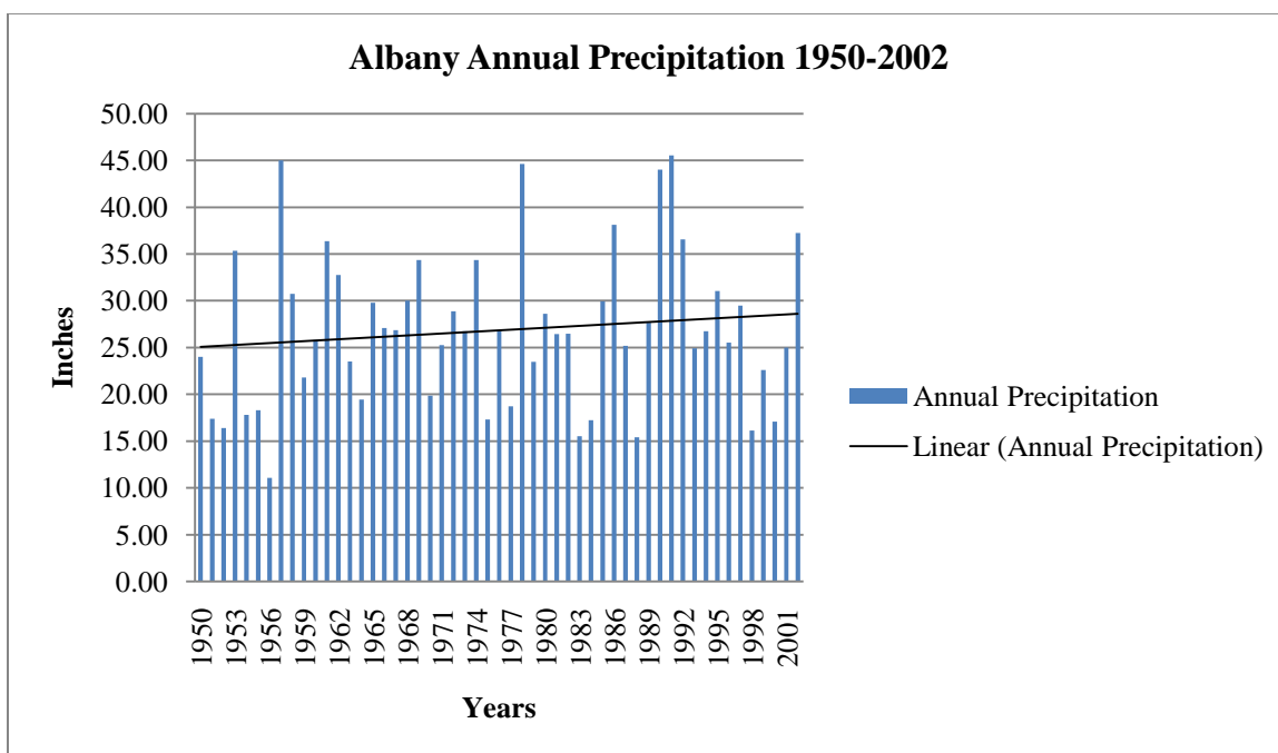
Figure 4. Albany Annual Precipitation for the Period 1950-2002. Trend is not significant ( p = 0.363 ), b = 0.068 .
