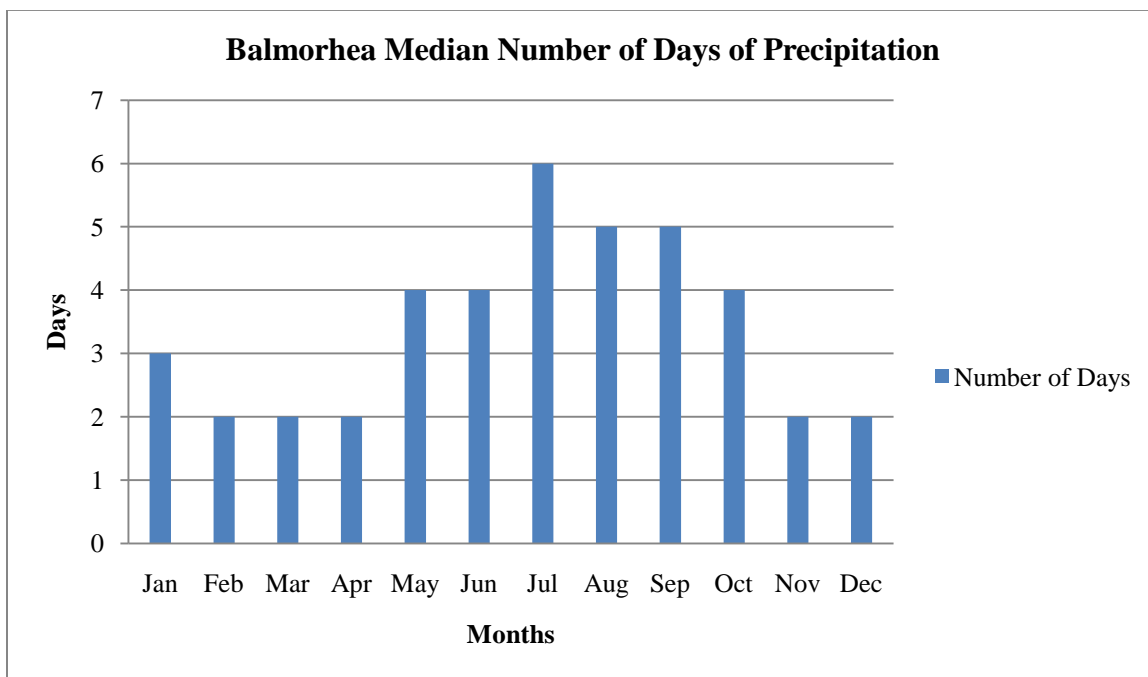
Figure 39. Balmorhea Median Monthly Number of Days of Precipitation for the Period 1923-2002.
