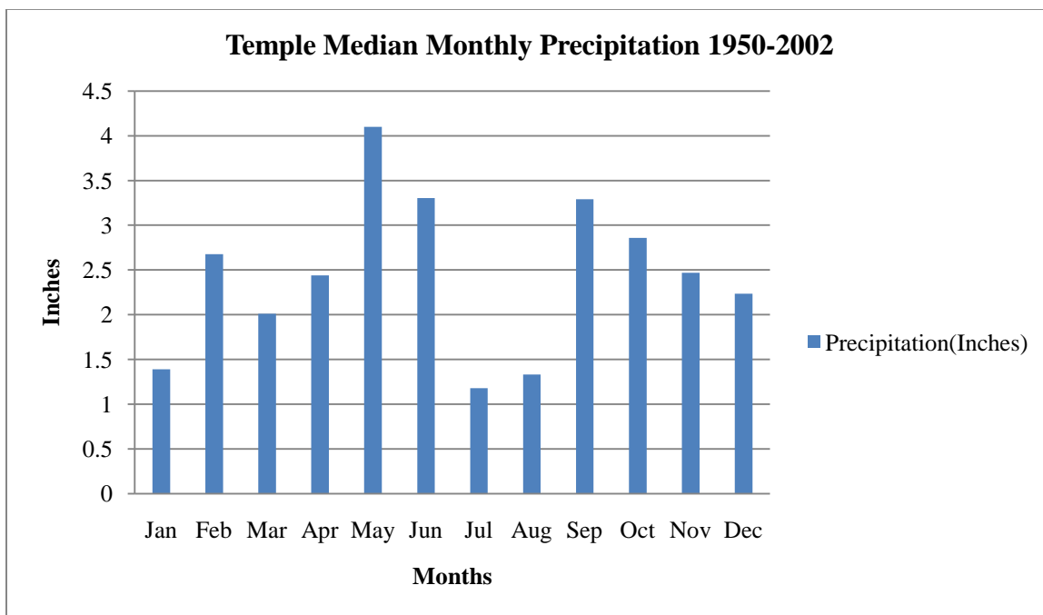
Figure 33. Temple Median Monthly Precipitation for the Period 1950-2002.
