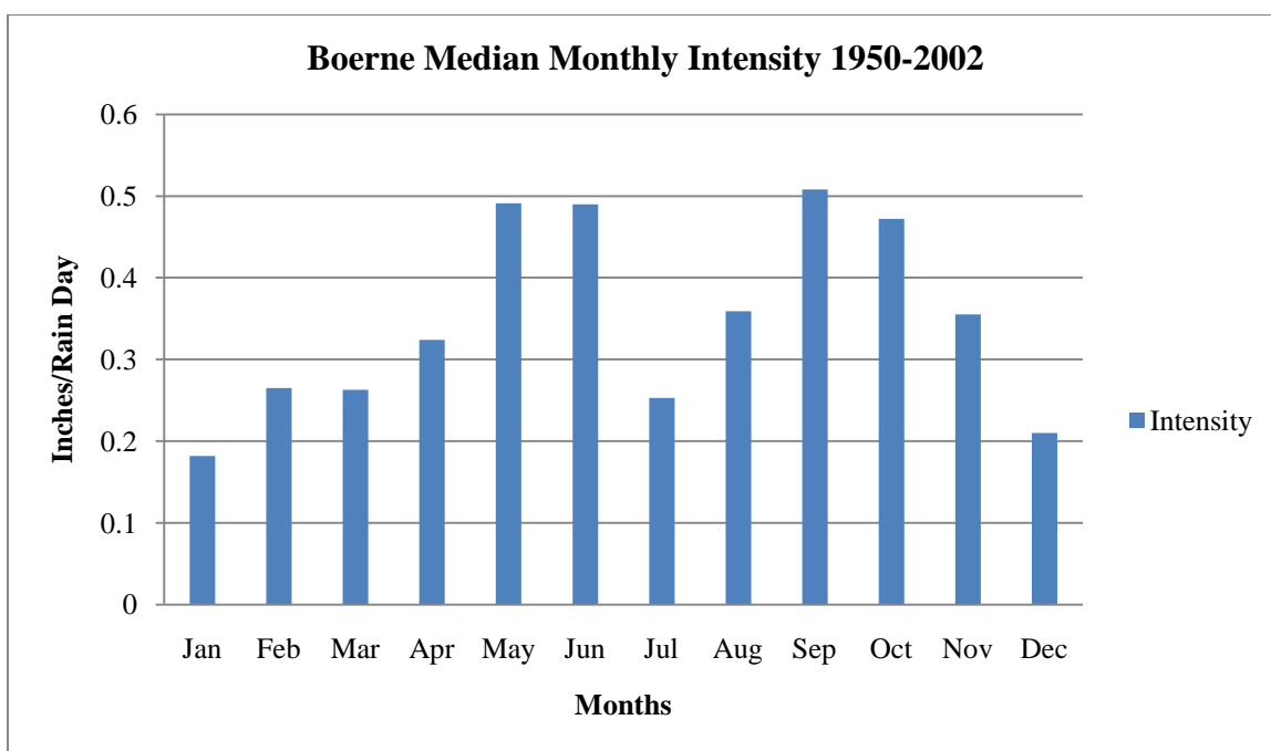
Figure 71. Boerne Median Monthly Intensity for the Period 1950-2002.
