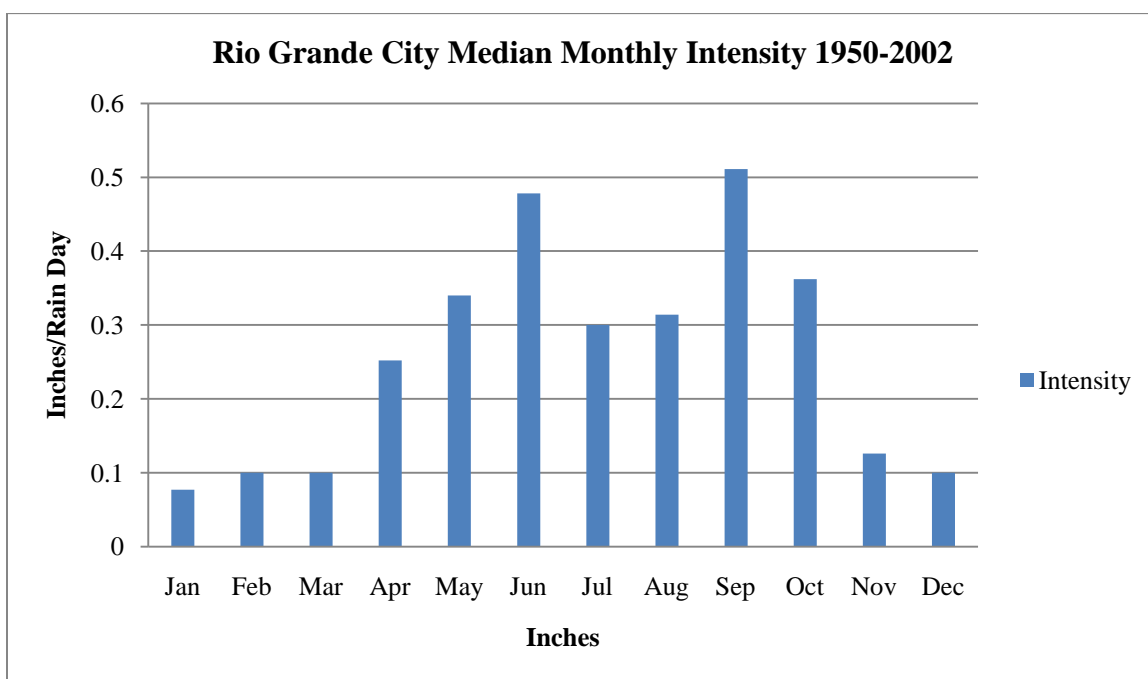
Figure 79. Rio Grande City Median Monthly Intensity for the Period 1950-2002.
