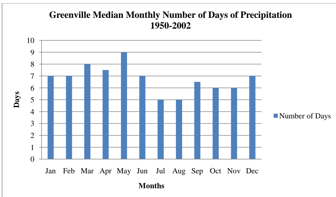
Figure 53. Greenville Median Monthly Number of Days of Precipitation for the Period 1950-2002.
