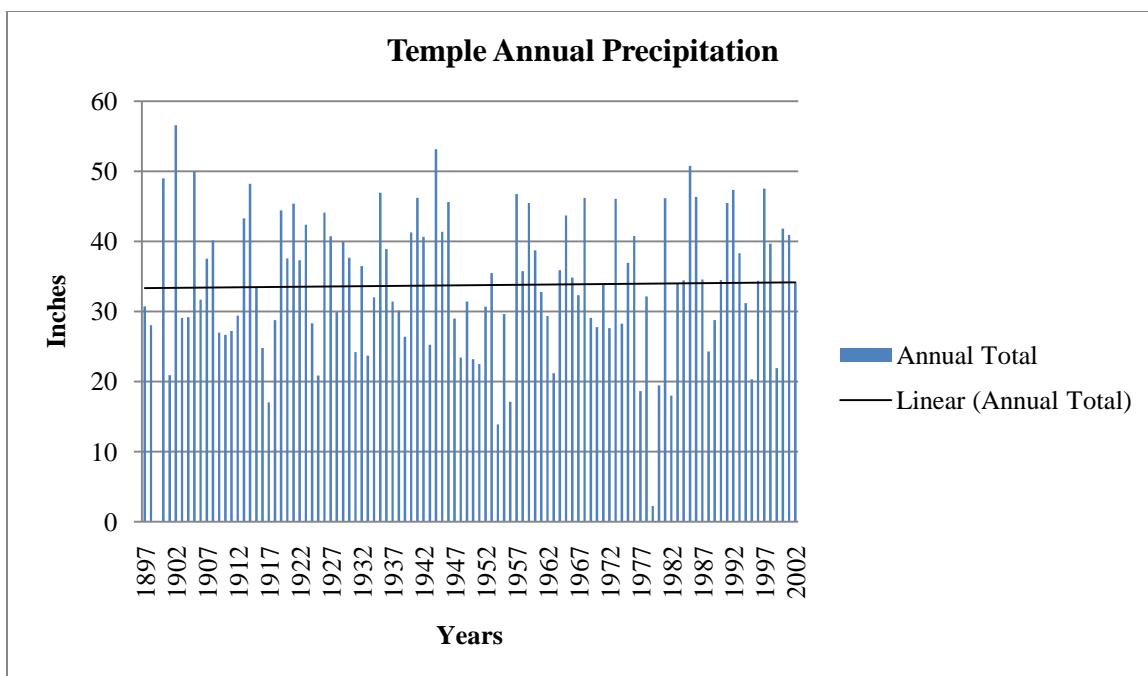
Figure 30. Temple Annual Precipitation for the Period 1897-2002. Trend is not significant ( p = 0.808 ), b = 0.008 .
