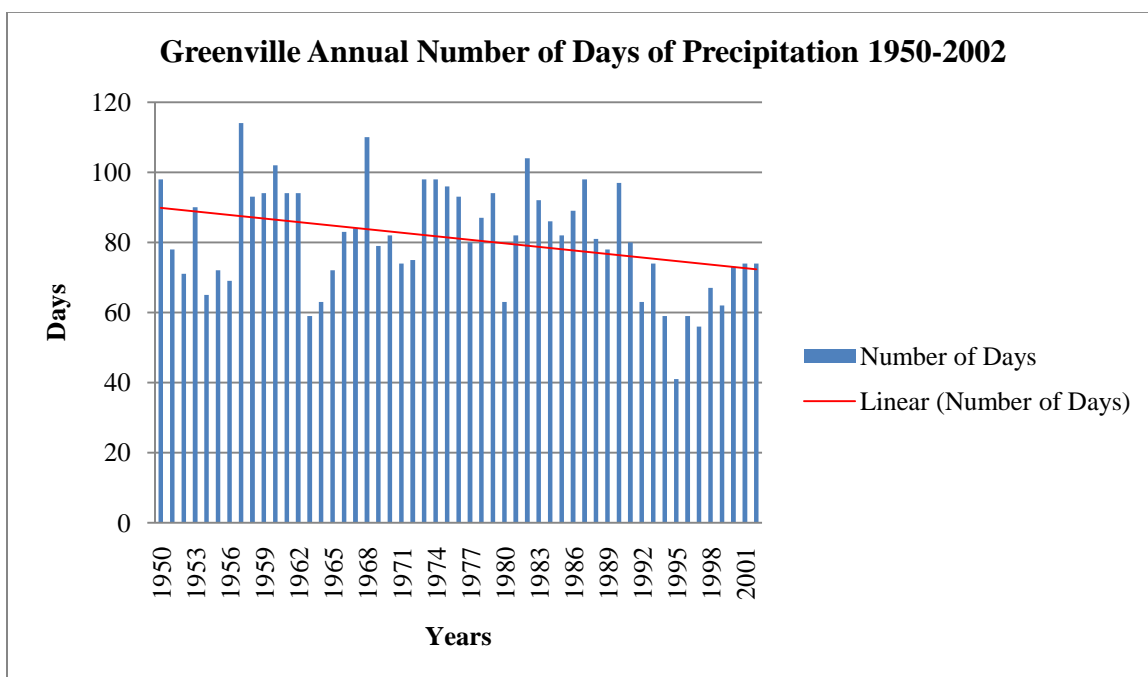
Figure 52. Greenville Annual Number of Days of Precipitation for the Period 1950-2002. Trend is significant ( p = 0.012 ), b = -0.337 .
