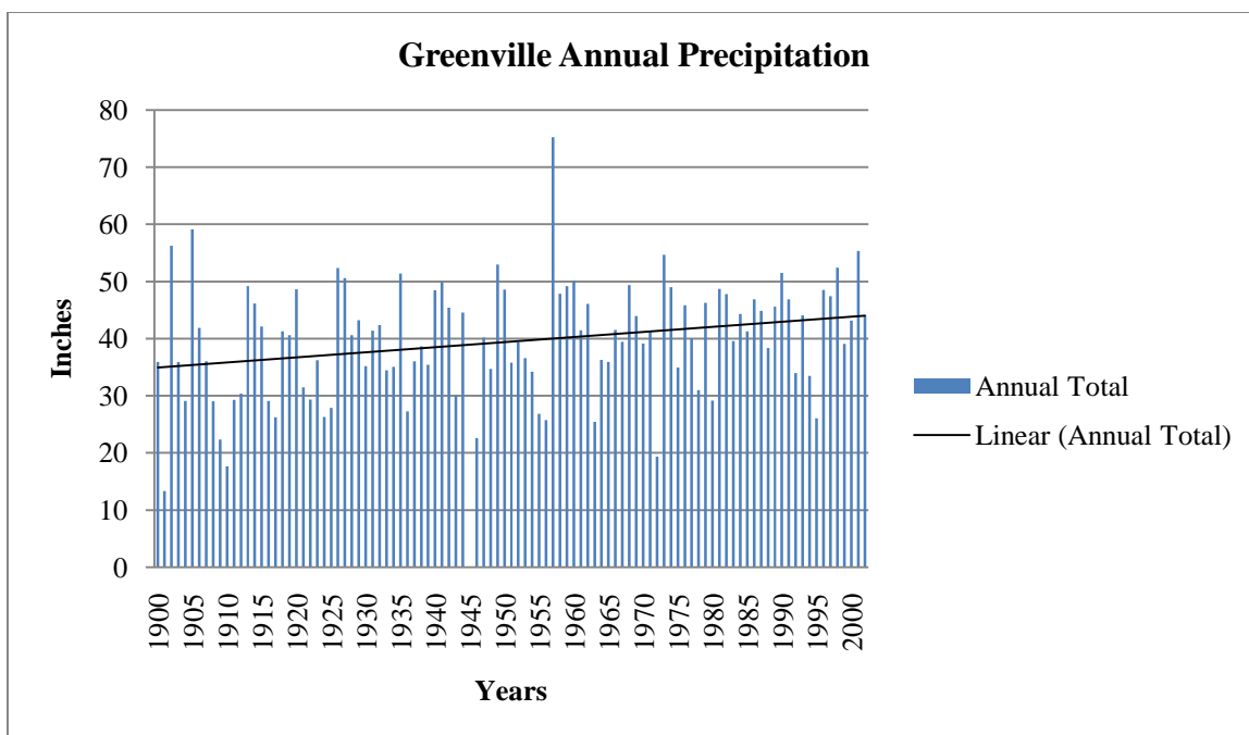
Figure 18. Greenville Annual Precipitation for the Period 1900-2002. Trend is significant ( p = 0.011 ), b = 0.089 .
