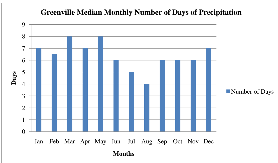
Figure 51. Greenville Median Monthly Number of Days of Precipitation for the Period 1900-2002.
