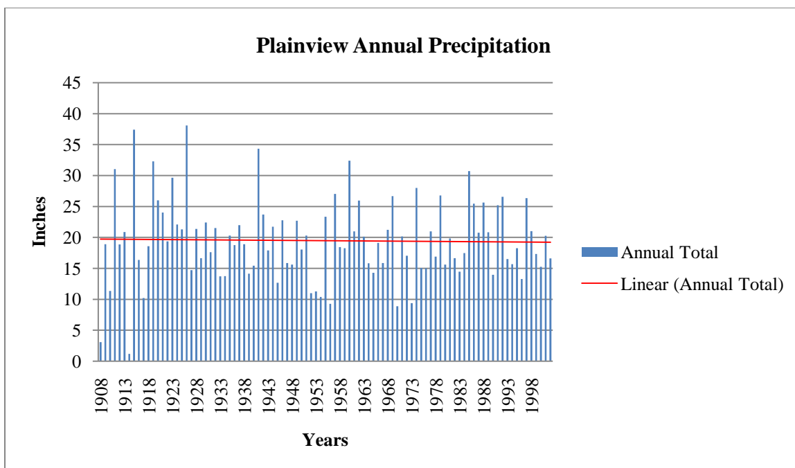
Figure 22. Plainview Annual Precipitation for the Period 1908-2002. Trend is not significant ( p = 0.831 ), b = -0.005 .
