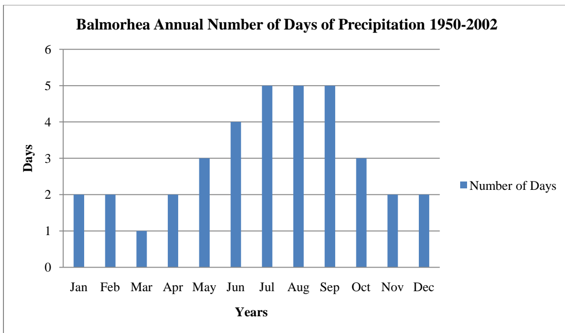
Figure 41. Balmorhea Median Monthly Number of Days of Precipitation for the Period 1950-2002.
