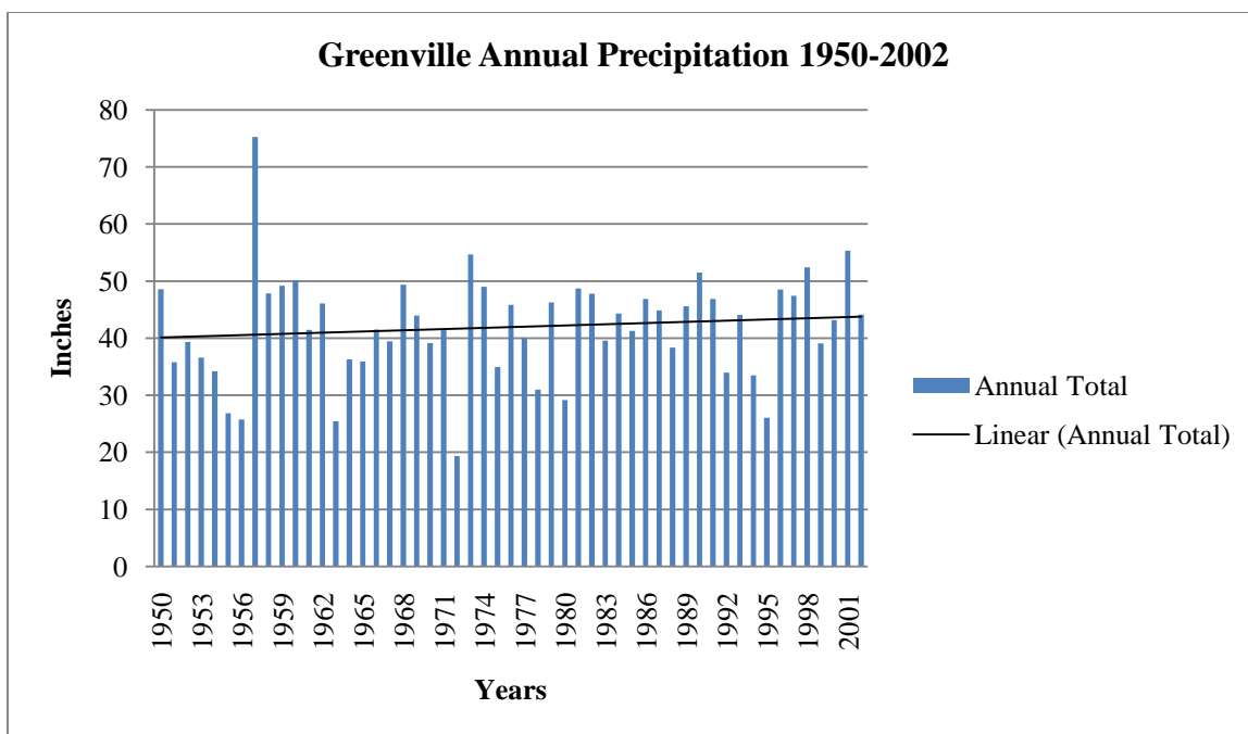
Figure 20. Greenville Annual Precipitation for the Period 1950-2002. Trend is not significant ( p = 0.399 ), b = 0.071 .
