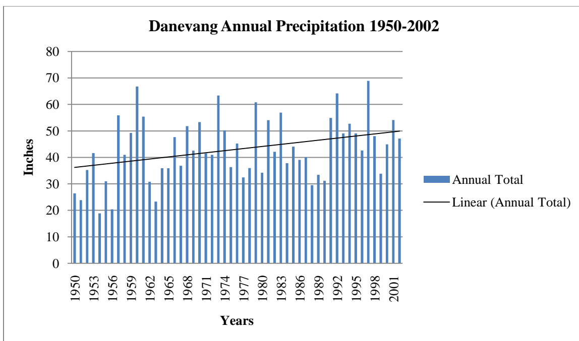
Figure 16. Danevang Annual Precipitation for the Period 1950-2002. Trend is significant ( p = 0.012 ), b = 0.263 .
