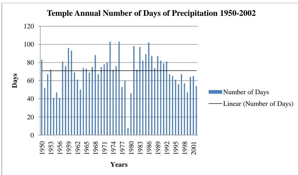
Figure 64. Temple Annual Number of Days of Precipitation for the Period 1950-2002. Trend is not significant ( p = 0.983 ), b = 0.004 .
