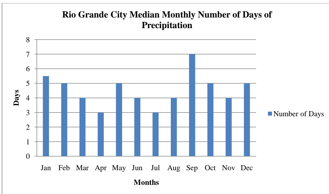
Figure 59. Rio Grande City Median Monthly Number of Days of Precipitation for the Period 1897-2002.
