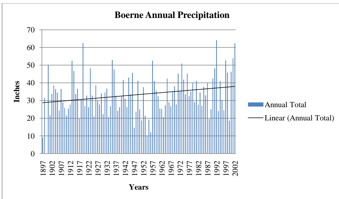
Figure 10. Boerne Annual Precipitation for the Period 1897-2002. Trend is significant ( p = 0.016 ), b = 0.088 .
