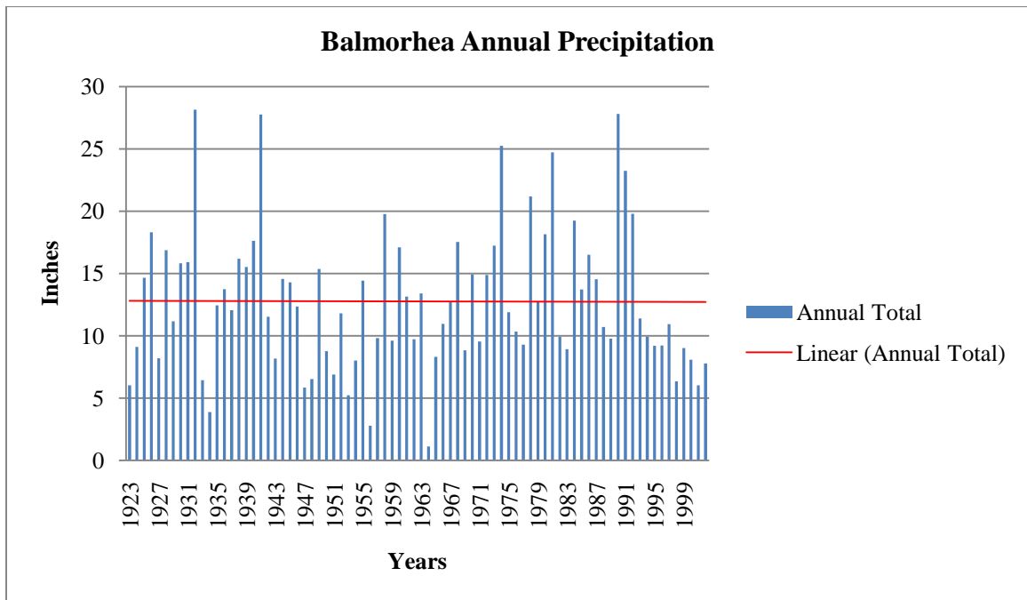
Figure 6. Balmorhea Annual Precipitation for the Period 1923-2002. Trend is not significant ( p = 0.960 ), b = -0.001 .
