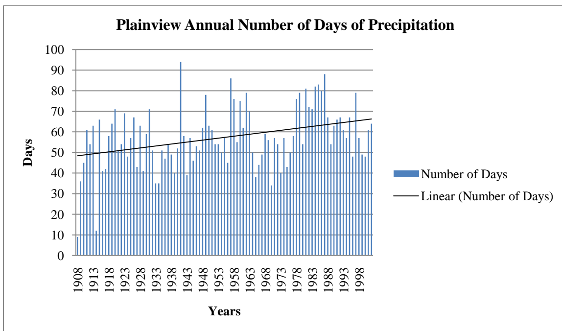
Figure 54. Plainview Annual Number of Days of Precipitation for the Period 1908-2002. Trend is significant ( p = 0.000 ), b = 0.190 .
