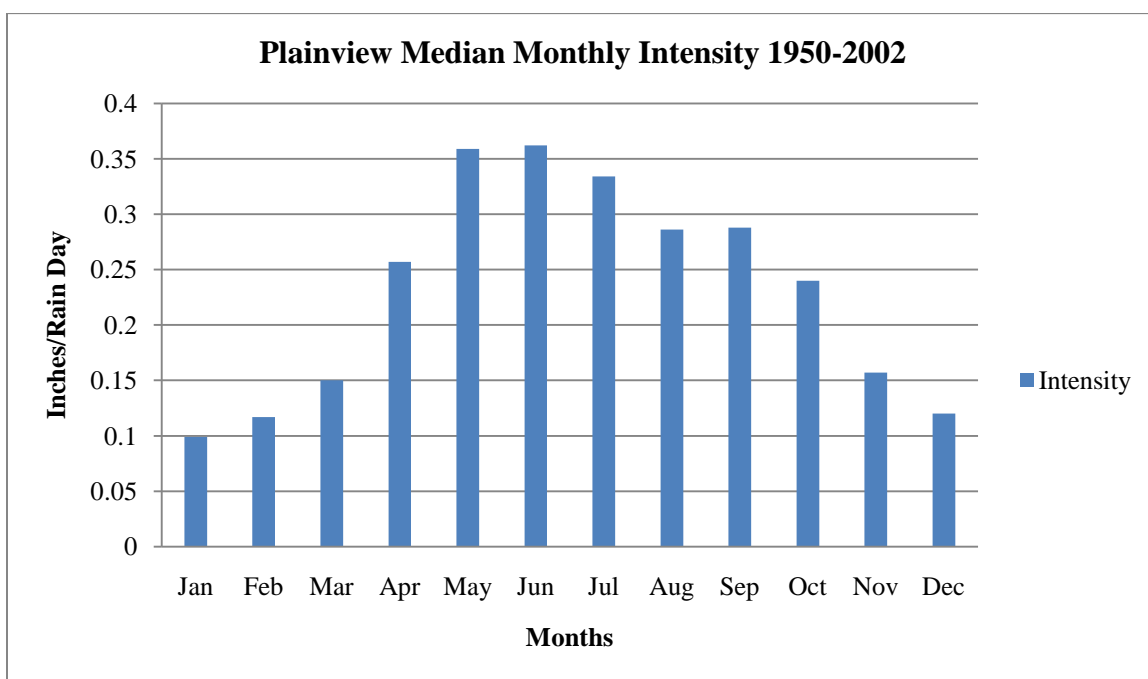
Figure 77. Plainview Median Monthly Intensity for the Period 1950-2002.
