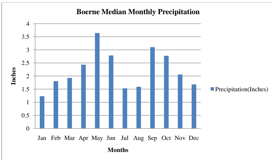
Figure 11. Boerne Median Monthly Precipitation for the Period 1897-2002.
