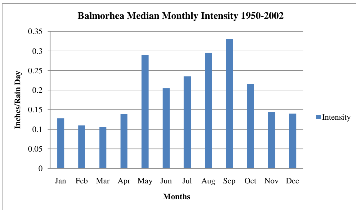
Figure 69. Balmorhea Median Monthly Intensity for the Period 1950-2002.
