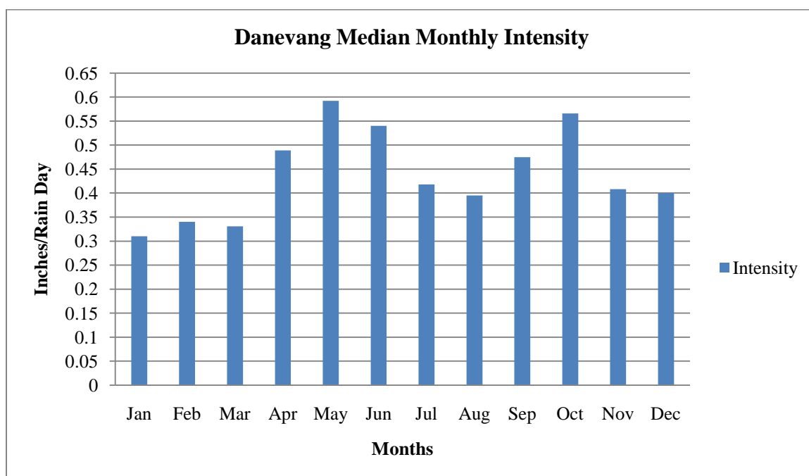
Figure 72. Danevang Median Monthly Intensity for the Period 1897-2002.
