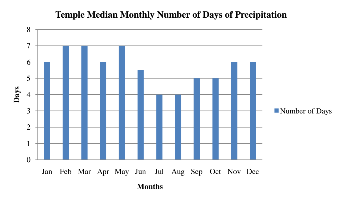
Figure 63. Temple Median Monthly Number of Days of Precipitation for the Period 1897-2002.
