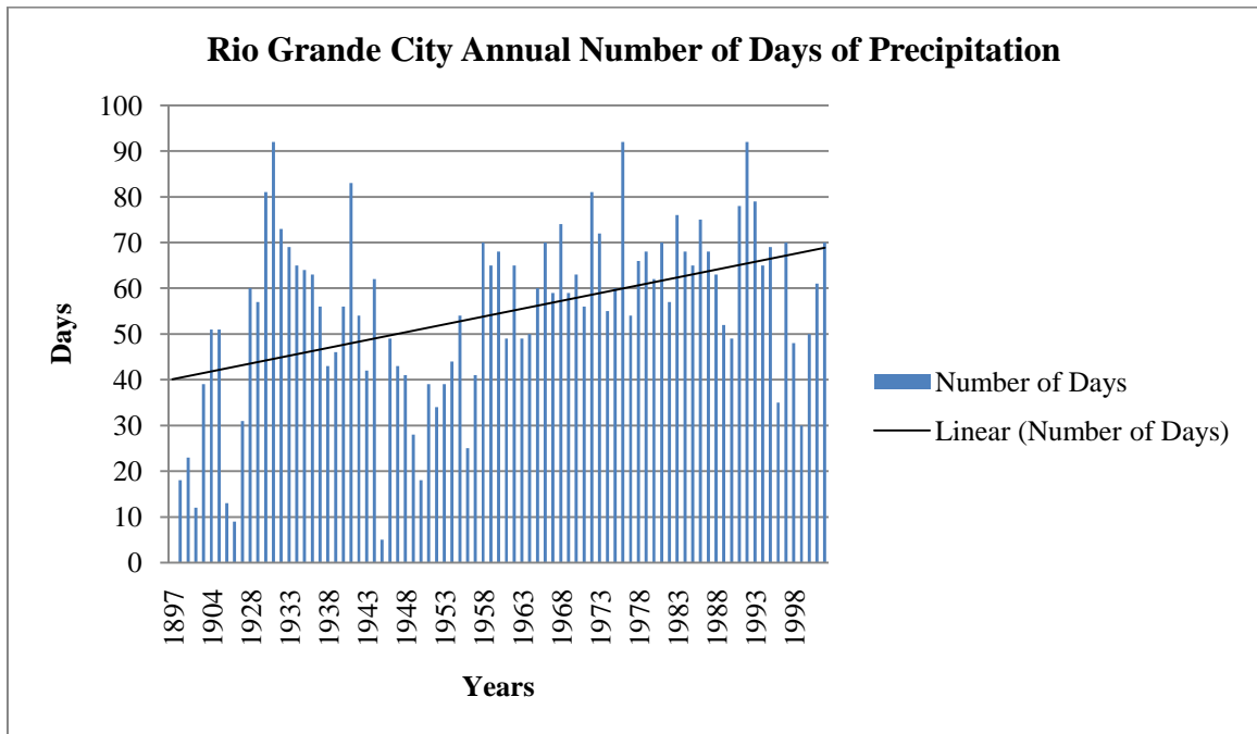
Figure 58. Rio Grande City Annual Number of Days of Precipitation for the Period 1897-2002. Trend is significant ( p = 0.000 ), b = 0.337 .
