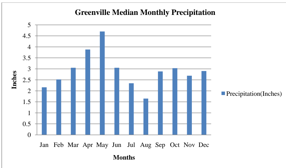
Figure 19. Greenville Median Monthly Precipitation for the Period 1900-2002.
