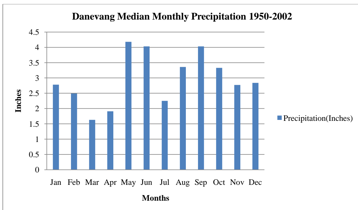
Figure 17. Danevang Median Monthly Precipitation for the Period 1950-2002.
