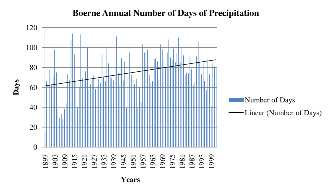
Figure 42. Boerne Annual Number of Days of Precipitation for the Period 1897-2002. Trend is significant ( p = 0.000 ), b = 0.250 .
