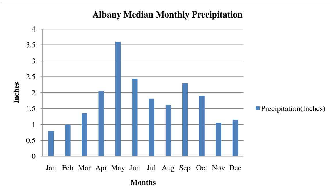
Figure 3. Albany Median Monthly Precipitation for the Period 1901-2002.
